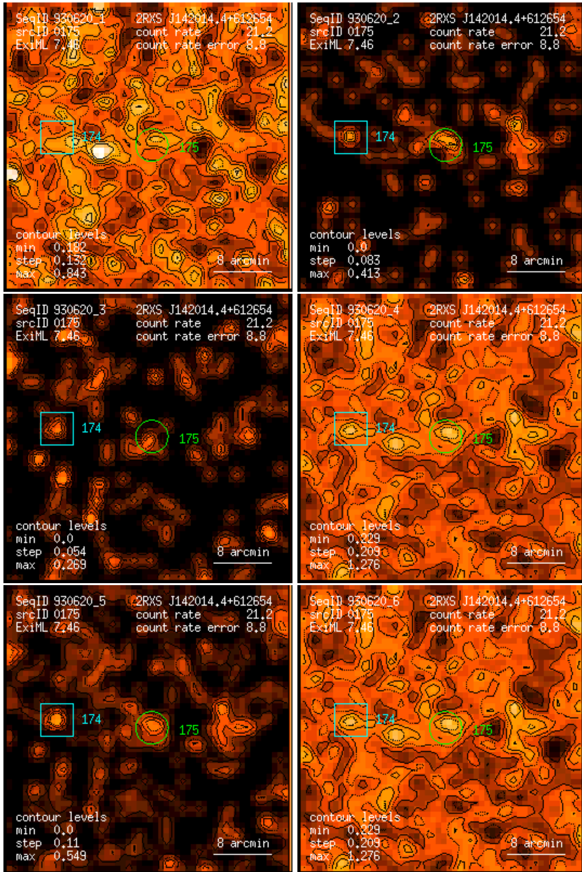
Figure 175: RASS 930620: detection 0175: band rate images, Gaussian filter: (1) PSPC channels 11 – 41, (2) 52 – 90, (3) 91 – 201, (4) 11 – 235, (5) 52 – 201, (6) 11 – 201. Broad band rates in counts/ks. Band rate contour levels in counts/ks/arcmin 2 .
