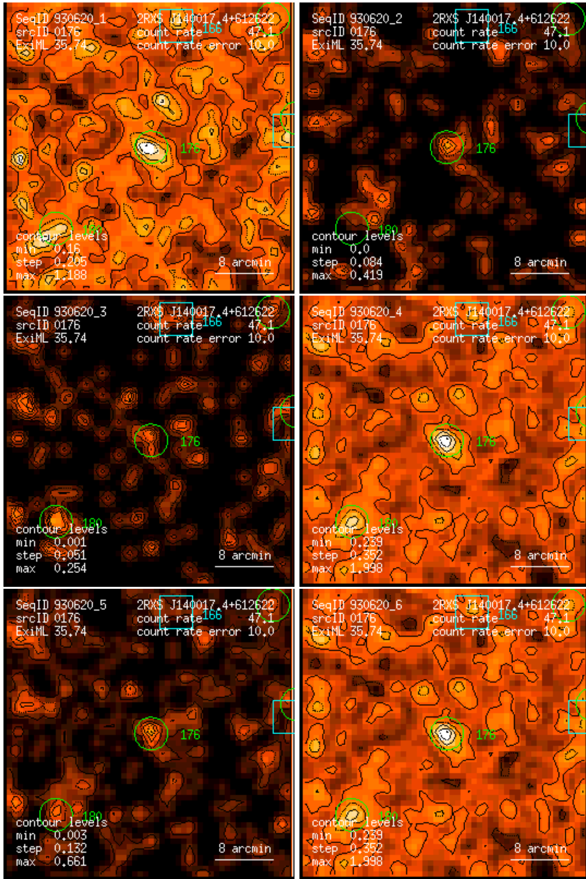
Figure 176: RASS 930620: detection 0176: band rate images, Gaussian filter: (1) PSPC channels 11 – 41, (2) 52 – 90, (3) 91 – 201, (4) 11 – 235, (5) 52 – 201, (6) 11 – 201. Broad band rates in counts/ks. Band rate contour levels in counts/ks/arcmin 2 .
