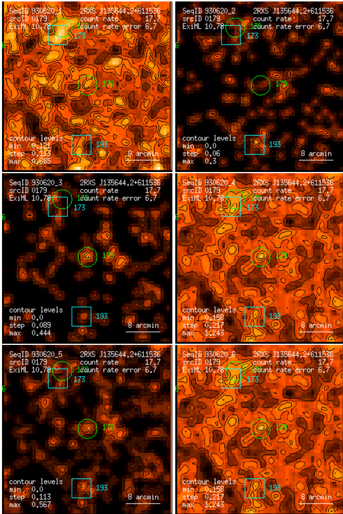
Figure 179: RASS 930620: detection 0179: band rate images, Gaussian filter: (1) PSPC channels 11 – 41, (2) 52 – 90, (3) 91 – 201, (4) 11 – 235, (5) 52 – 201, (6) 11 – 201. Broad band rates in counts/ks. Band rate contour levels in counts/ks/arcmin 2 .
