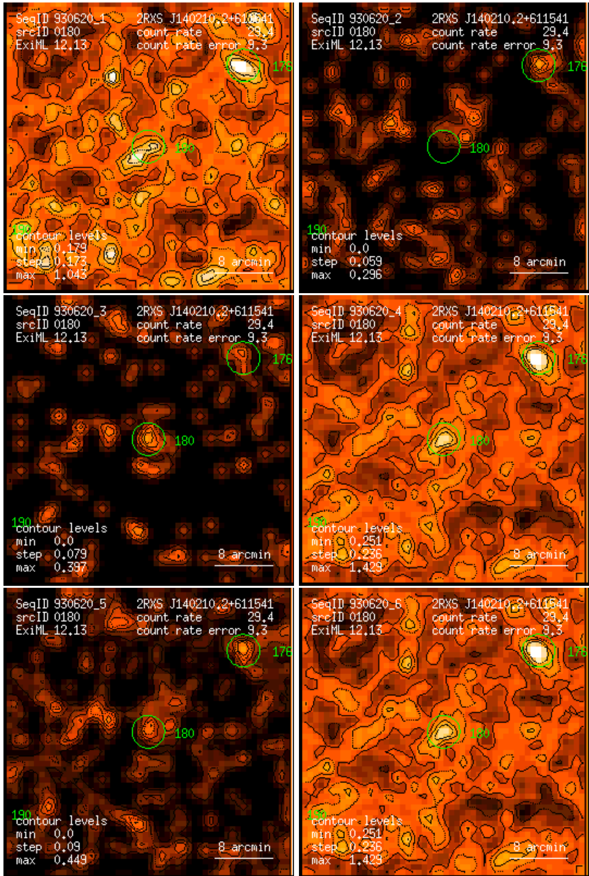
Figure 180: RASS 930620: detection 0180: band rate images, Gaussian filter: (1) PSPC channels 11 – 41, (2) 52 – 90, (3) 91 – 201, (4) 11 – 235, (5) 52 – 201, (6) 11 – 201. Broad band rates in counts/ks. Band rate contour levels in counts/ks/arcmin 2 .
