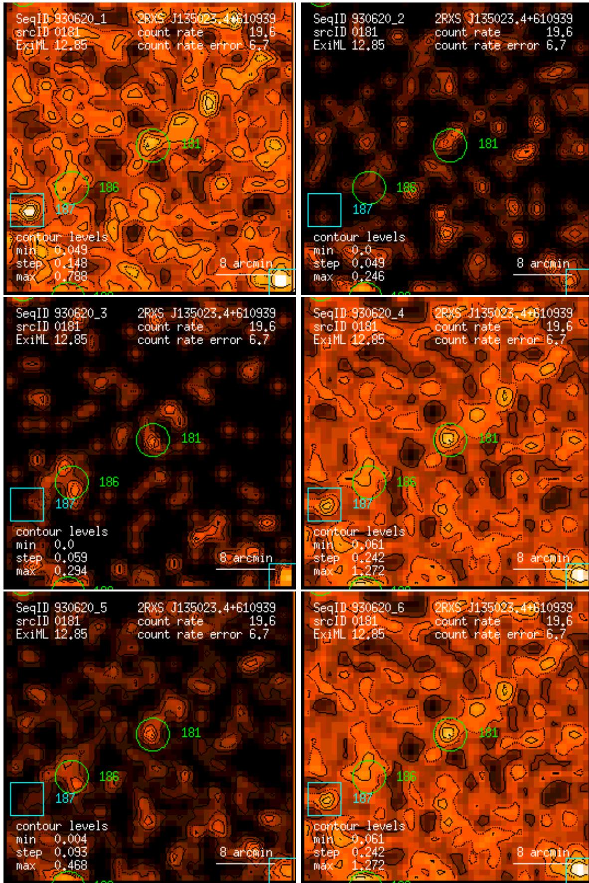
Figure 181: RASS 930620: detection 0181: band rate images, Gaussian filter: (1) PSPC channels 11 – 41, (2) 52 – 90, (3) 91 – 201, (4) 11 – 235, (5) 52 – 201, (6) 11 – 201. Broad band rates in counts/ks. Band rate contour levels in counts/ks/arcmin 2 .
