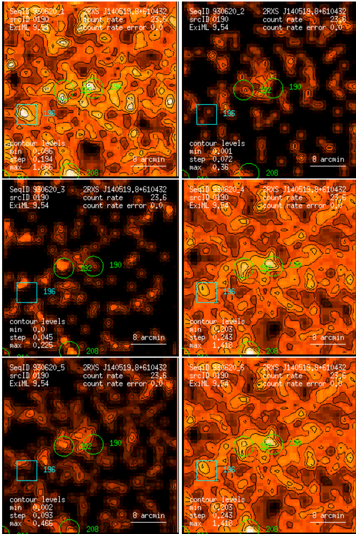
Figure 190: RASS 930620: detection 0190: band rate images, Gaussian filter: (1) PSPC channels 11 – 41, (2) 52 – 90, (3) 91 – 201, (4) 11 – 235, (5) 52 – 201, (6) 11 – 201. Broad band rates in counts/ks. Band rate contour levels in counts/ks/arcmin 2 .
