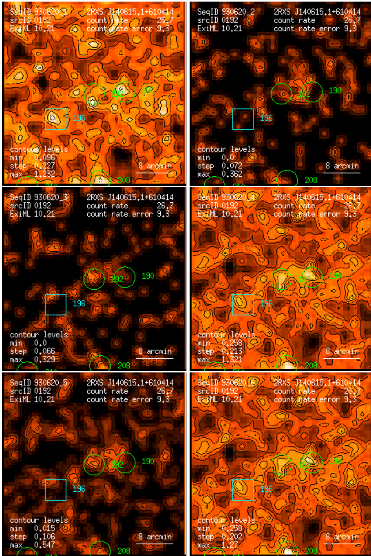
Figure 192: RASS 930620: detection 0192: band rate images, Gaussian filter: (1) PSPC channels 11 – 41, (2) 52 – 90, (3) 91 – 201, (4) 11 – 235, (5) 52 – 201, (6) 11 – 201. Broad band rates in counts/ks. Band rate contour levels in counts/ks/arcmin 2 .
