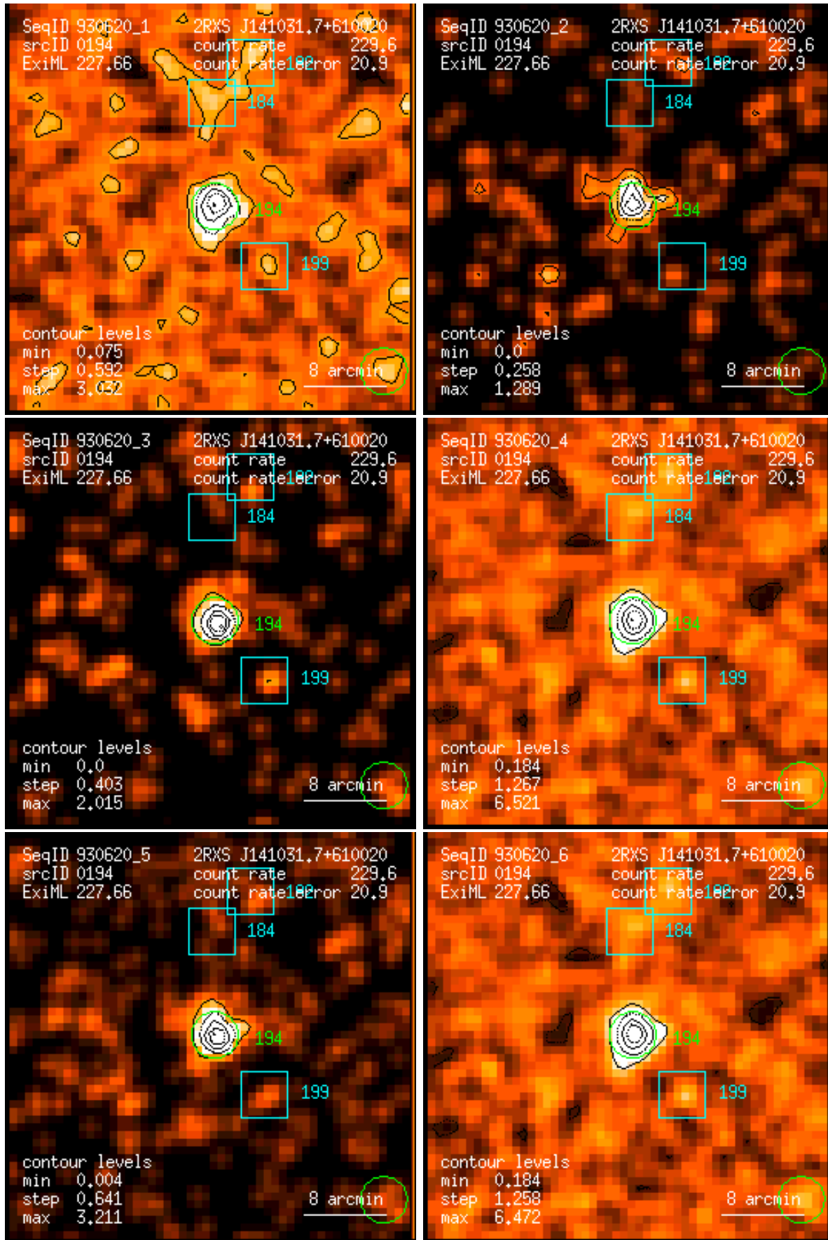
Figure 194: RASS 930620: detection 0194: band rate images, Gaussian filter: (1) PSPC channels 11 – 41, (2) 52 – 90, (3) 91 – 201, (4) 11 – 235, (5) 52 – 201, (6) 11 – 201. Broad band rates in counts/ks. Band rate contour levels in counts/ks/arcmin 2 .
