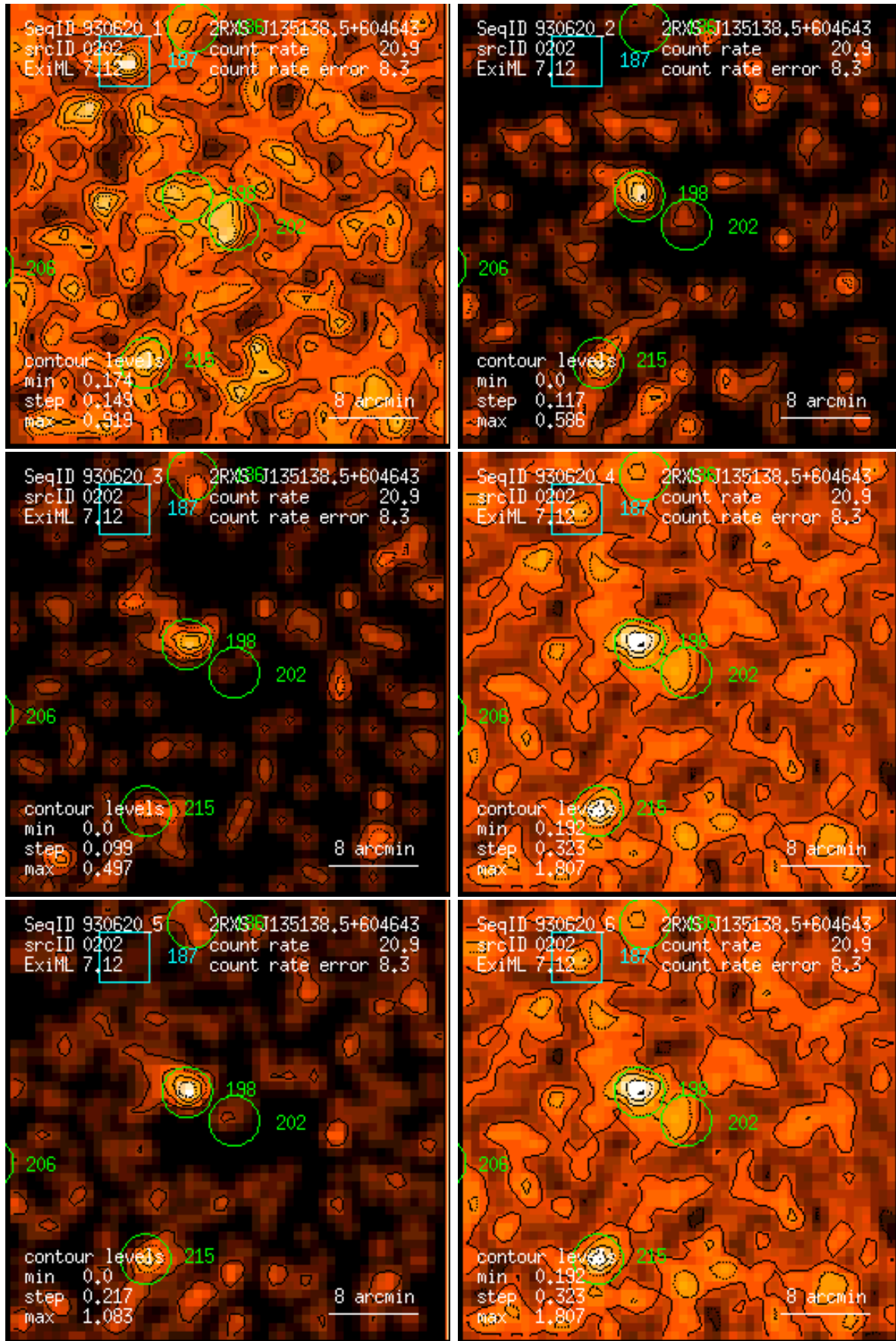
Figure 202: RASS 930620: detection 0202: band rate images, Gaussian filter: (1) PSPC channels 11 – 41, (2) 52 – 90, (3) 91 – 201, (4) 11 – 235, (5) 52 – 201, (6) 11 – 201. Broad band rates in counts/ks. Band rate contour levels in counts/ks/arcmin 2 .
