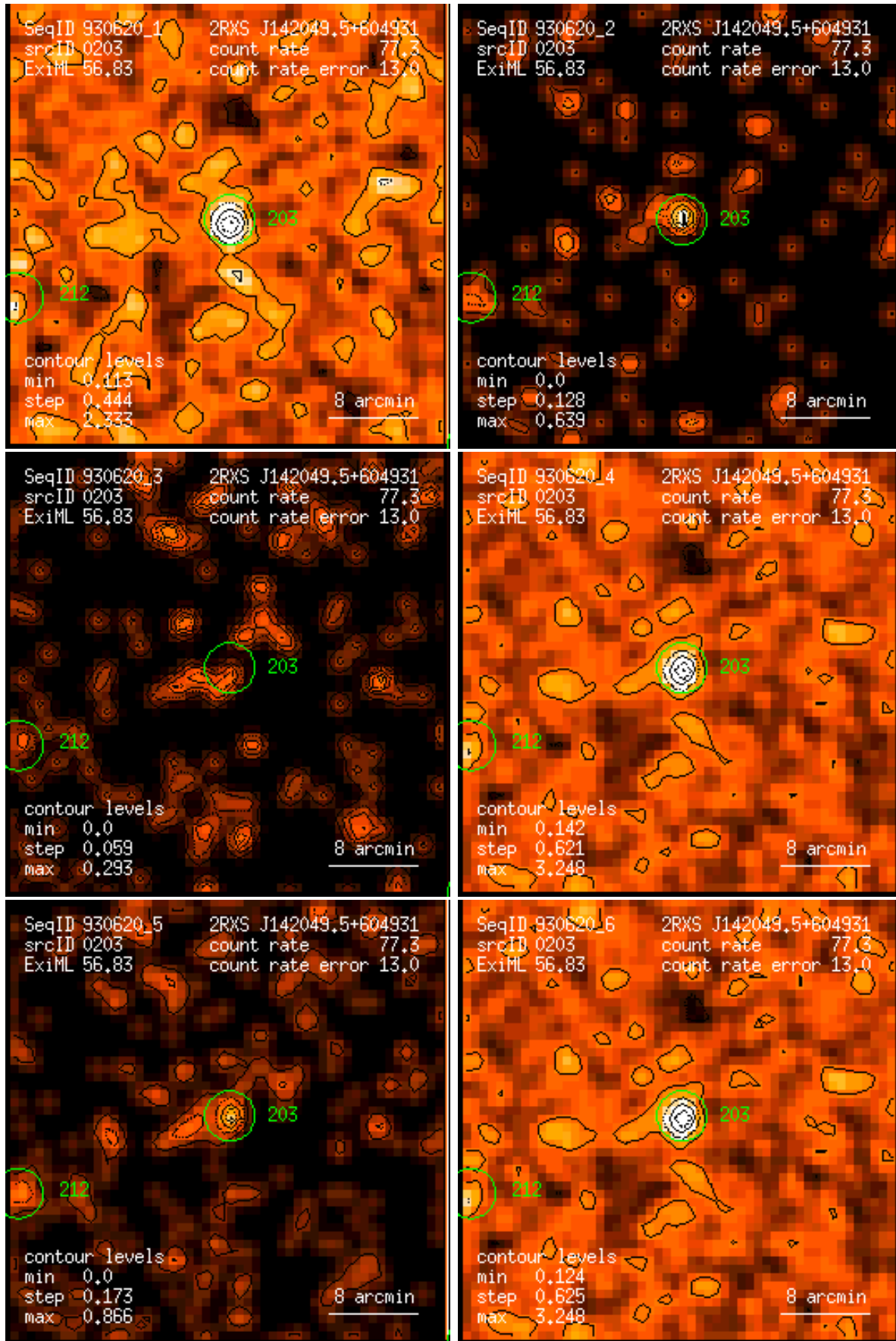
Figure 203: RASS 930620: detection 0203: band rate images, Gaussian filter: (1) PSPC channels 11 – 41, (2) 52 – 90, (3) 91 – 201, (4) 11 – 235, (5) 52 – 201, (6) 11 – 201. Broad band rates in counts/ks. Band rate contour levels in counts/ks/arcmin 2 .
