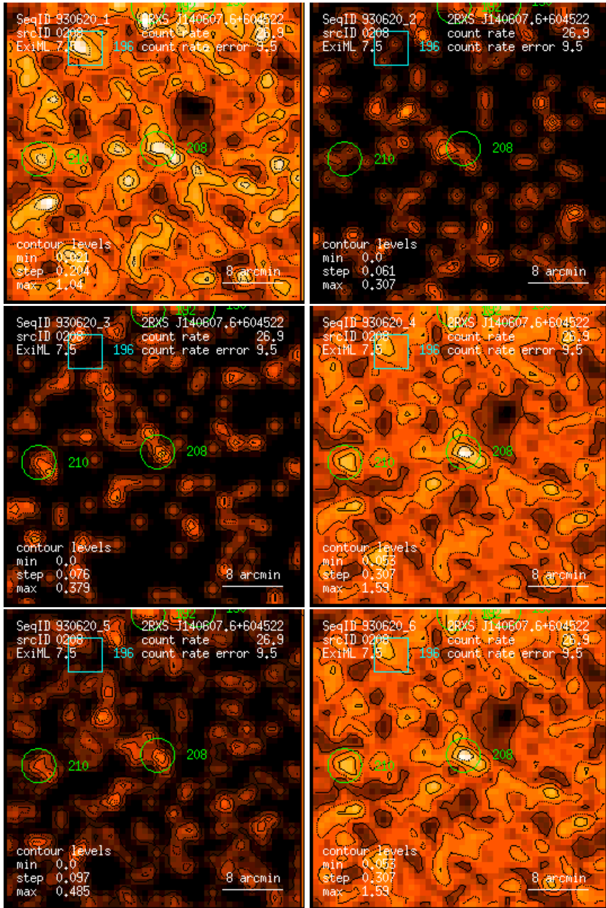
Figure 208: RASS 930620: detection 0208: band rate images, Gaussian filter: (1) PSPC channels 11 – 41, (2) 52 – 90, (3) 91 – 201, (4) 11 – 235, (5) 52 – 201, (6) 11 – 201. Broad band rates in counts/ks. Band rate contour levels in counts/ks/arcmin 2 .
