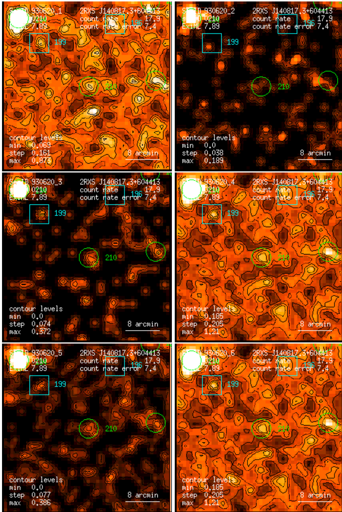
Figure 210: RASS 930620: detection 0210: band rate images, Gaussian filter: (1) PSPC channels 11 – 41, (2) 52 – 90, (3) 91 – 201, (4) 11 – 235, (5) 52 – 201, (6) 11 – 201. Broad band rates in counts/ks. Band rate contour levels in counts/ks/arcmin 2 .
