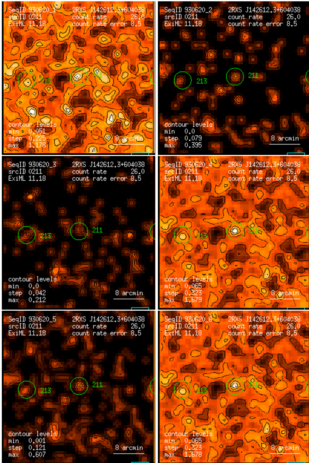
Figure 211: RASS 930620: detection 0211: band rate images, Gaussian filter: (1) PSPC channels 11 – 41, (2) 52 – 90, (3) 91 – 201, (4) 11 – 235, (5) 52 – 201, (6) 11 – 201. Broad band rates in counts/ks. Band rate contour levels in counts/ks/arcmin 2 .
