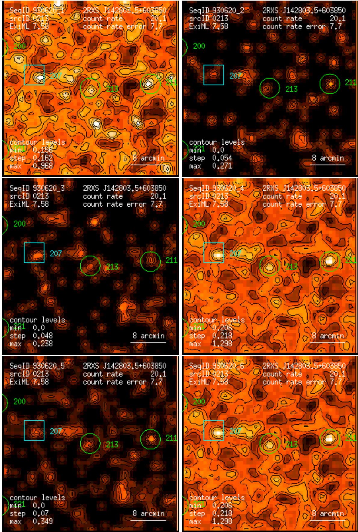
Figure 213: RASS 930620: detection 0213: band rate images, Gaussian filter: (1) PSPC channels 11 – 41, (2) 52 – 90, (3) 91 – 201, (4) 11 – 235, (5) 52 – 201, (6) 11 – 201. Broad band rates in counts/ks. Band rate contour levels in counts/ks/arcmin 2 .
