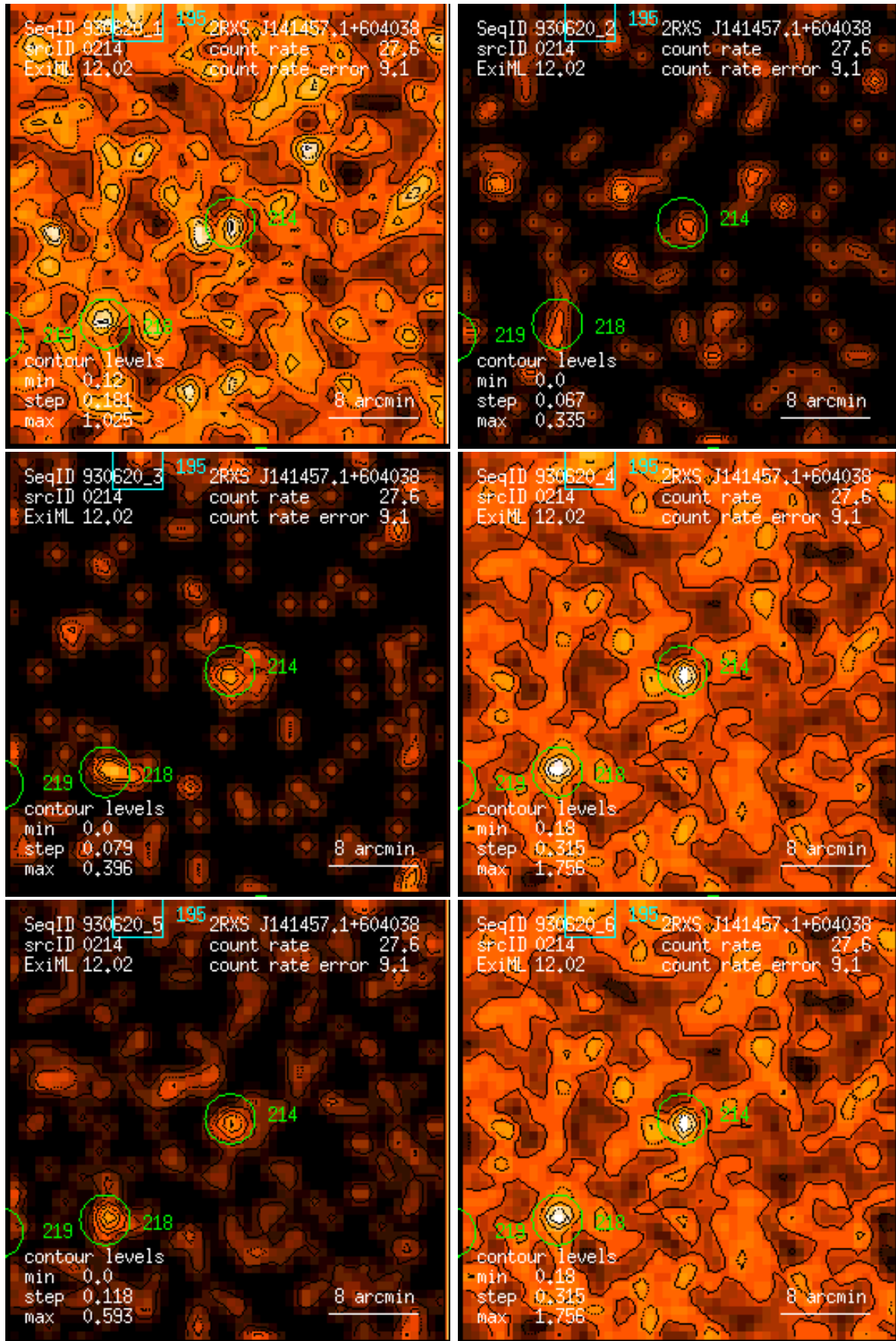
Figure 214: RASS 930620: detection 0214: band rate images, Gaussian filter: (1) PSPC channels 11 – 41, (2) 52 – 90, (3) 91 – 201, (4) 11 – 235, (5) 52 – 201, (6) 11 – 201. Broad band rates in counts/ks. Band rate contour levels in counts/ks/arcmin 2 .
