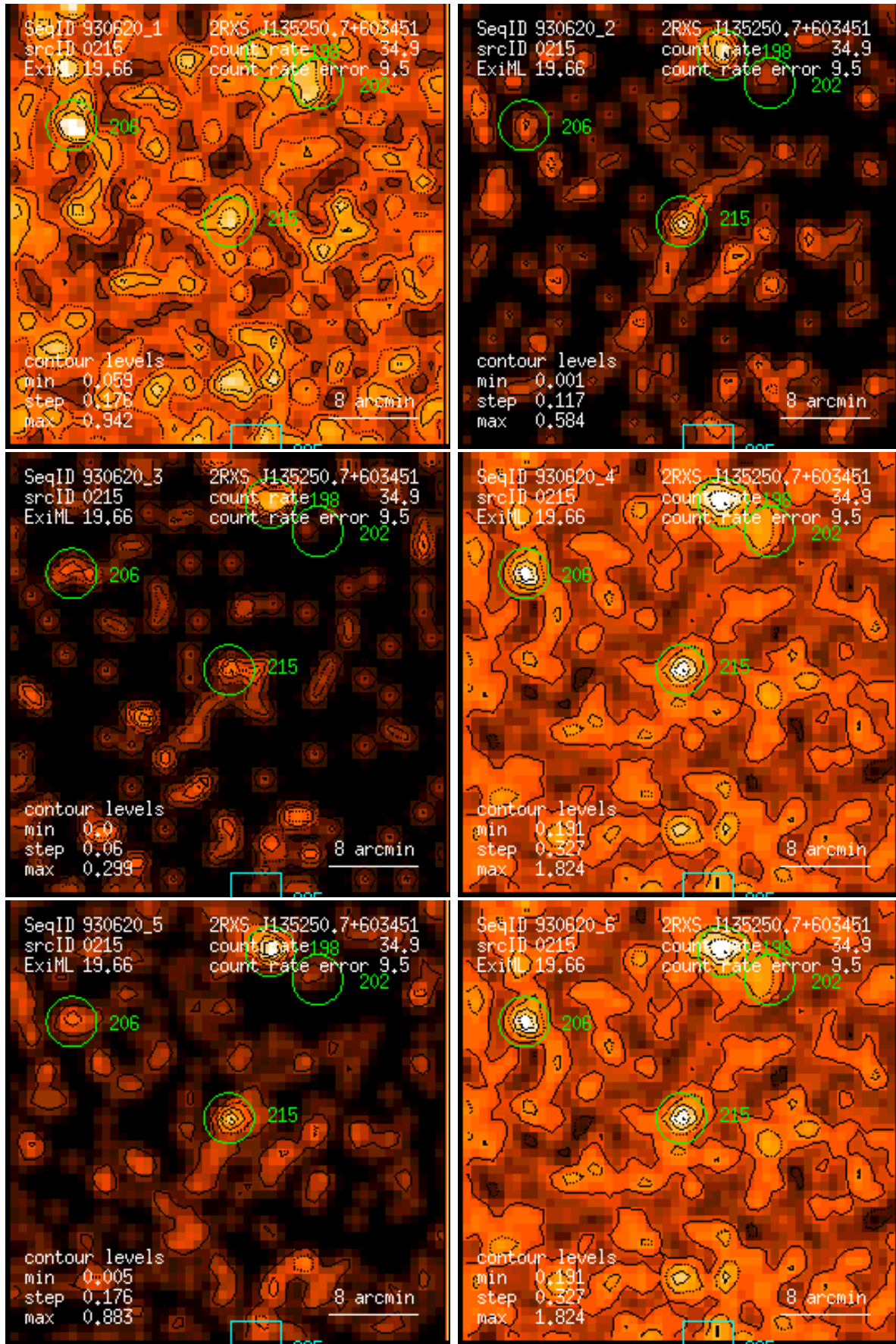
Figure 215: RASS 930620: detection 0215: band rate images, Gaussian filter: (1) PSPC channels 11 – 41, (2) 52 – 90, (3) 91 – 201, (4) 11 – 235, (5) 52 – 201, (6) 11 – 201. Broad band rates in counts/ks. Band rate contour levels in counts/ks/arcmin 2 .
