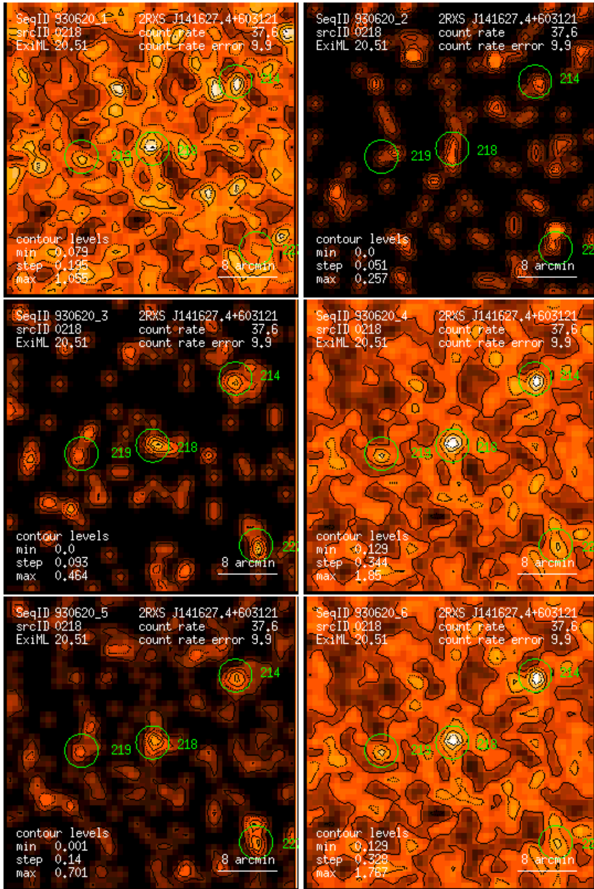
Figure 218: RASS 930620: detection 0218: band rate images, Gaussian filter: (1) PSPC channels 11 – 41, (2) 52 – 90, (3) 91 – 201, (4) 11 – 235, (5) 52 – 201, (6) 11 – 201. Broad band rates in counts/ks. Band rate contour levels in counts/ks/arcmin 2 .
