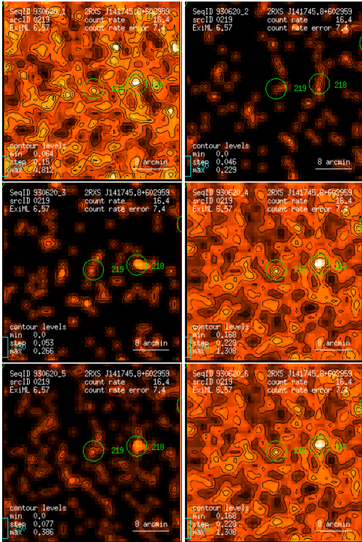
Figure 219: RASS 930620: detection 0219: band rate images, Gaussian filter: (1) PSPC channels 11 – 41, (2) 52 – 90, (3) 91 – 201, (4) 11 – 235, (5) 52 – 201, (6) 11 – 201. Broad band rates in counts/ks. Band rate contour levels in counts/ks/arcmin 2 .
