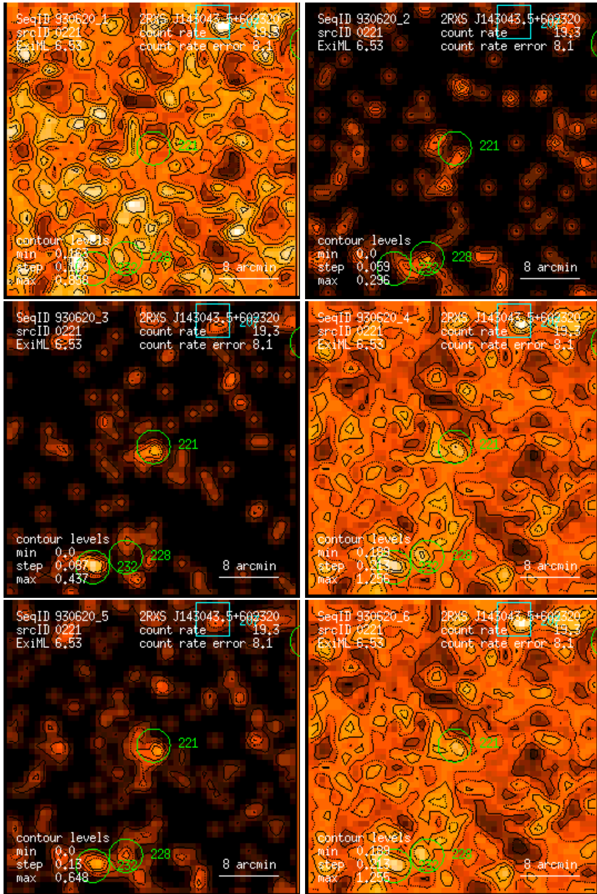
Figure 221: RASS 930620: detection 0221: band rate images, Gaussian filter: (1) PSPC channels 11 – 41, (2) 52 – 90, (3) 91 – 201, (4) 11 – 235, (5) 52 – 201, (6) 11 – 201. Broad band rates in counts/ks. Band rate contour levels in counts/ks/arcmin 2 .
