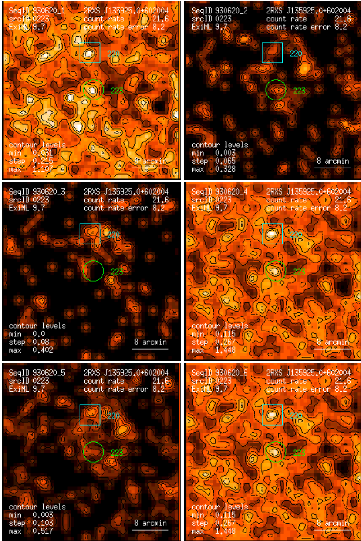
Figure 223: RASS 930620: detection 0223: band rate images, Gaussian filter: (1) PSPC channels 11 – 41, (2) 52 – 90, (3) 91 – 201, (4) 11 – 235, (5) 52 – 201, (6) 11 – 201. Broad band rates in counts/ks. Band rate contour levels in counts/ks/arcmin 2 .
