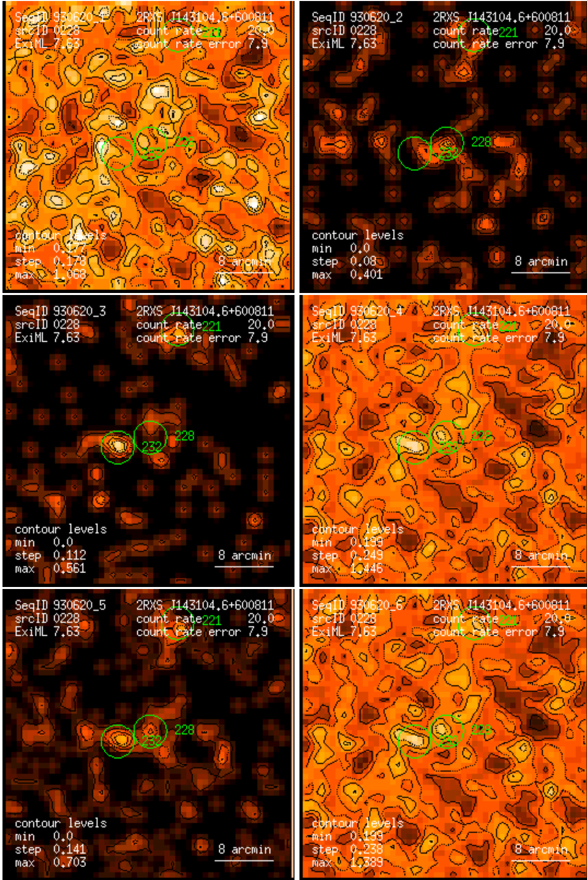
Figure 228: RASS 930620: detection 0228: band rate images, Gaussian filter: (1) PSPC channels 11 – 41, (2) 52 – 90, (3) 91 – 201, (4) 11 – 235, (5) 52 – 201, (6) 11 – 201. Broad band rates in counts/ks. Band rate contour levels in counts/ks/arcmin 2 .
