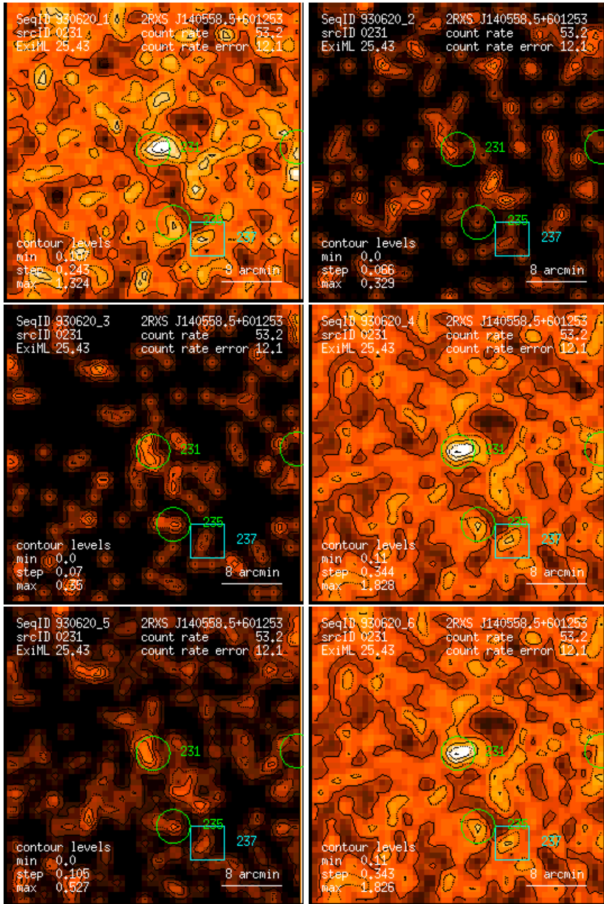
Figure 231: RASS 930620: detection 0231: band rate images, Gaussian filter: (1) PSPC channels 11 – 41, (2) 52 – 90, (3) 91 – 201, (4) 11 – 235, (5) 52 – 201, (6) 11 – 201. Broad band rates in counts/ks. Band rate contour levels in counts/ks/arcmin 2 .
