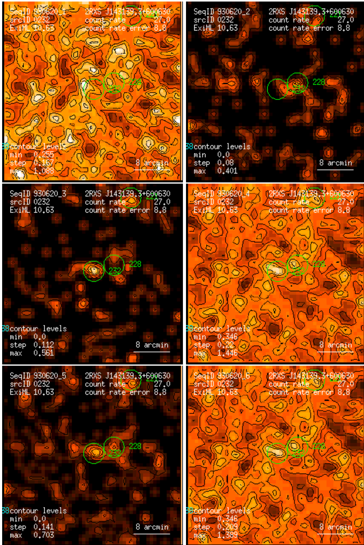
Figure 232: RASS 930620: detection 0232: band rate images, Gaussian filter: (1) PSPC channels 11 – 41, (2) 52 – 90, (3) 91 – 201, (4) 11 – 235, (5) 52 – 201, (6) 11 – 201. Broad band rates in counts/ks. Band rate contour levels in counts/ks/arcmin 2 .
