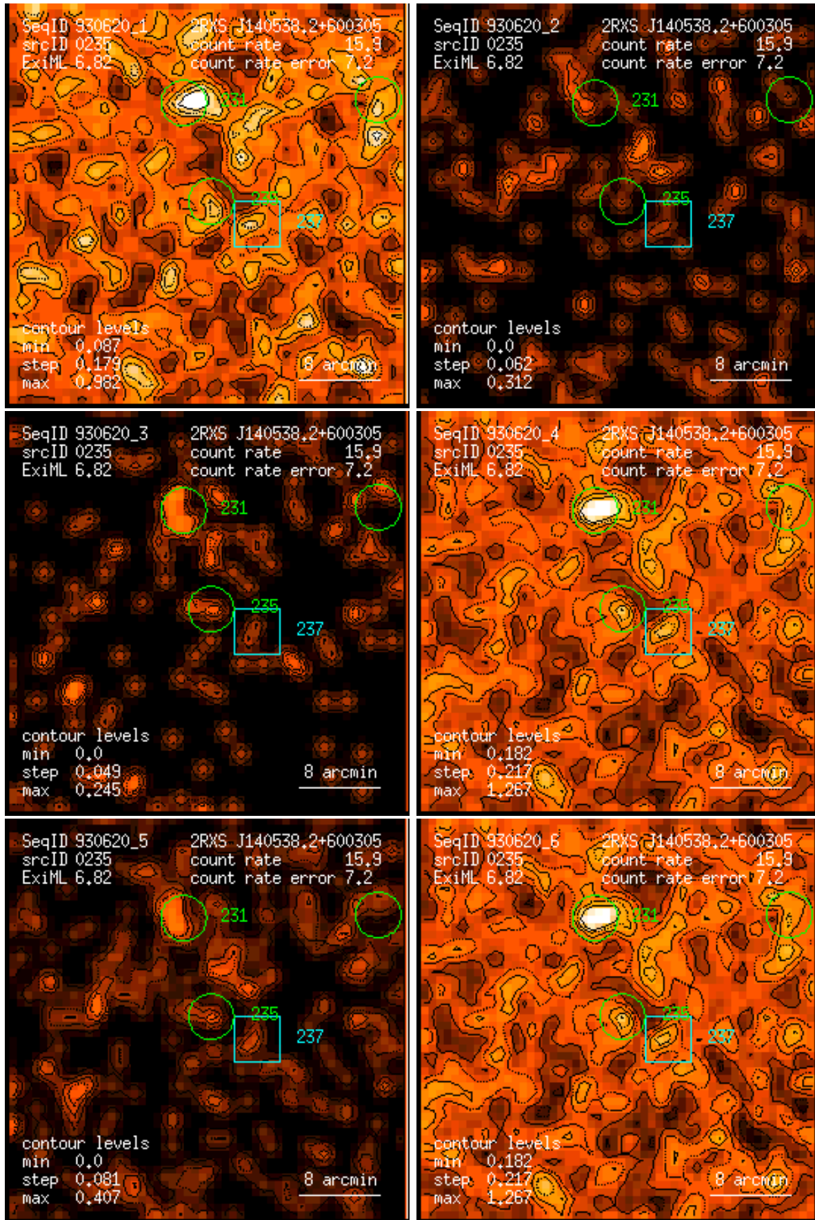
Figure 235: RASS 930620: detection 0235: band rate images, Gaussian filter: (1) PSPC channels 11 – 41, (2) 52 – 90, (3) 91 – 201, (4) 11 – 235, (5) 52 – 201, (6) 11 – 201. Broad band rates in counts/ks. Band rate contour levels in counts/ks/arcmin 2 .
