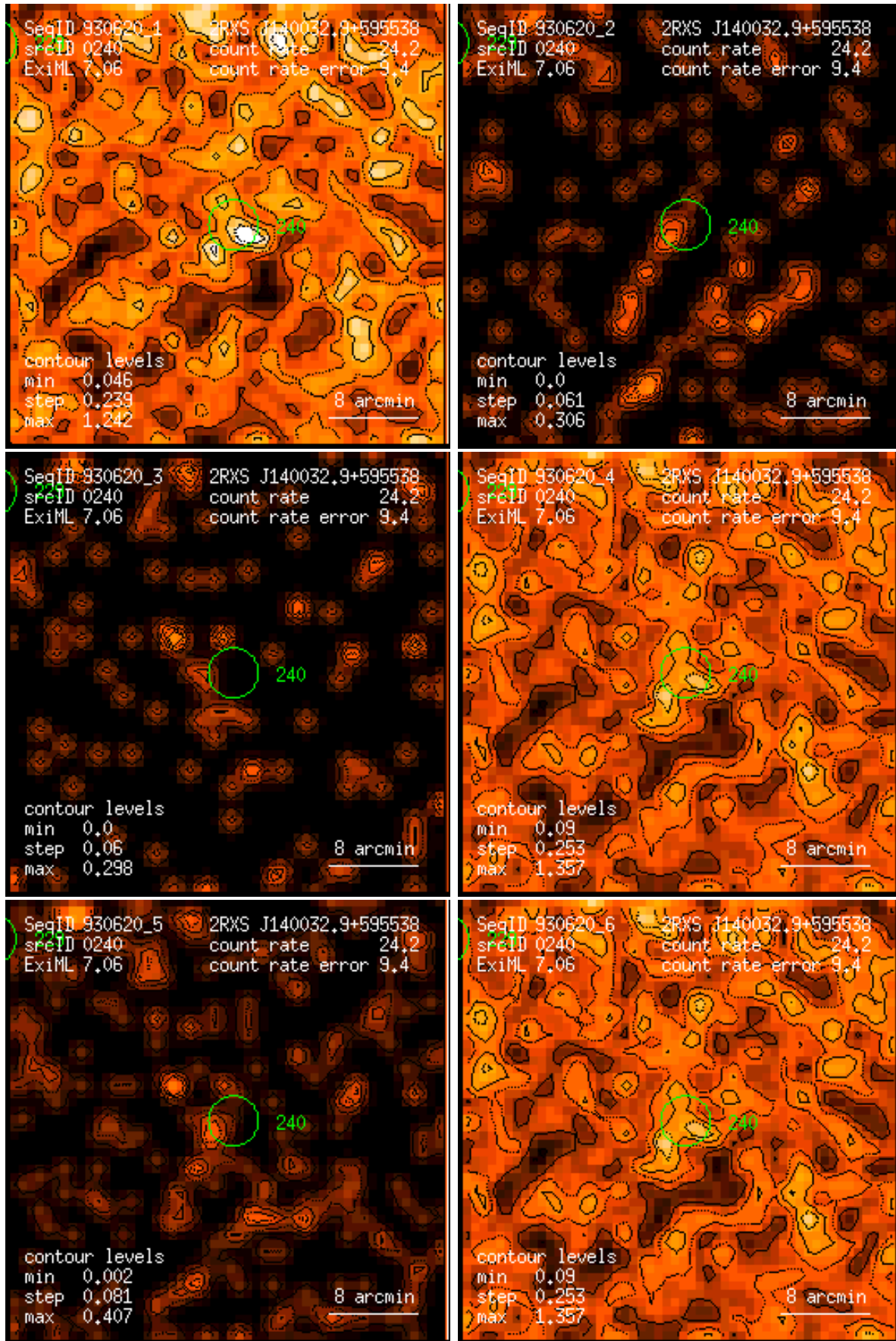
Figure 240: RASS 930620: detection 0240: band rate images, Gaussian filter: (1) PSPC channels 11 – 41, (2) 52 – 90, (3) 91 – 201, (4) 11 – 235, (5) 52 – 201, (6) 11 – 201. Broad band rates in counts/ks. Band rate contour levels in counts/ks/arcmin 2 .
