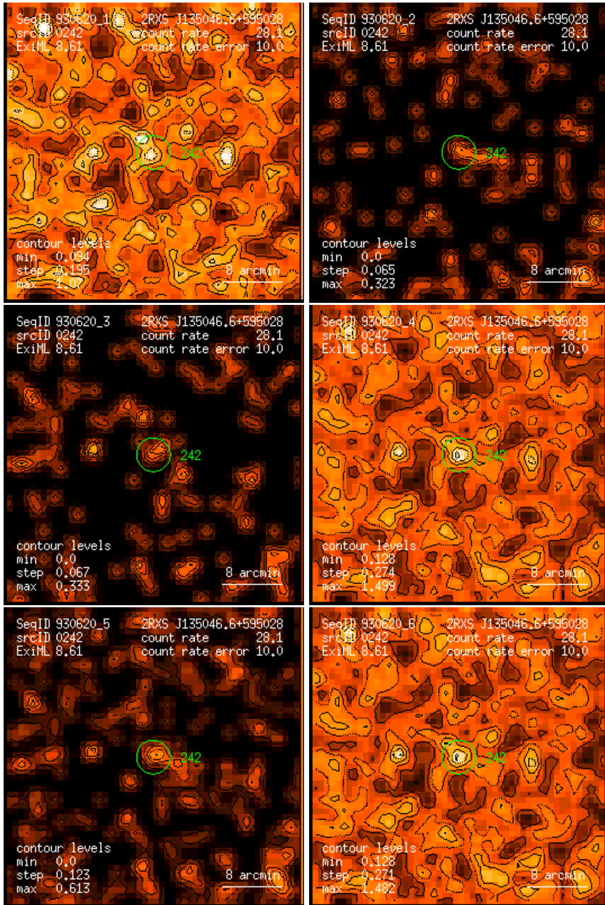
Figure 242: RASS 930620: detection 0242: band rate images, Gaussian filter: (1) PSPC channels 11 – 41, (2) 52 – 90, (3) 91 – 201, (4) 11 – 235, (5) 52 – 201, (6) 11 – 201. Broad band rates in counts/ks. Band rate contour levels in counts/ks/arcmin 2 .
