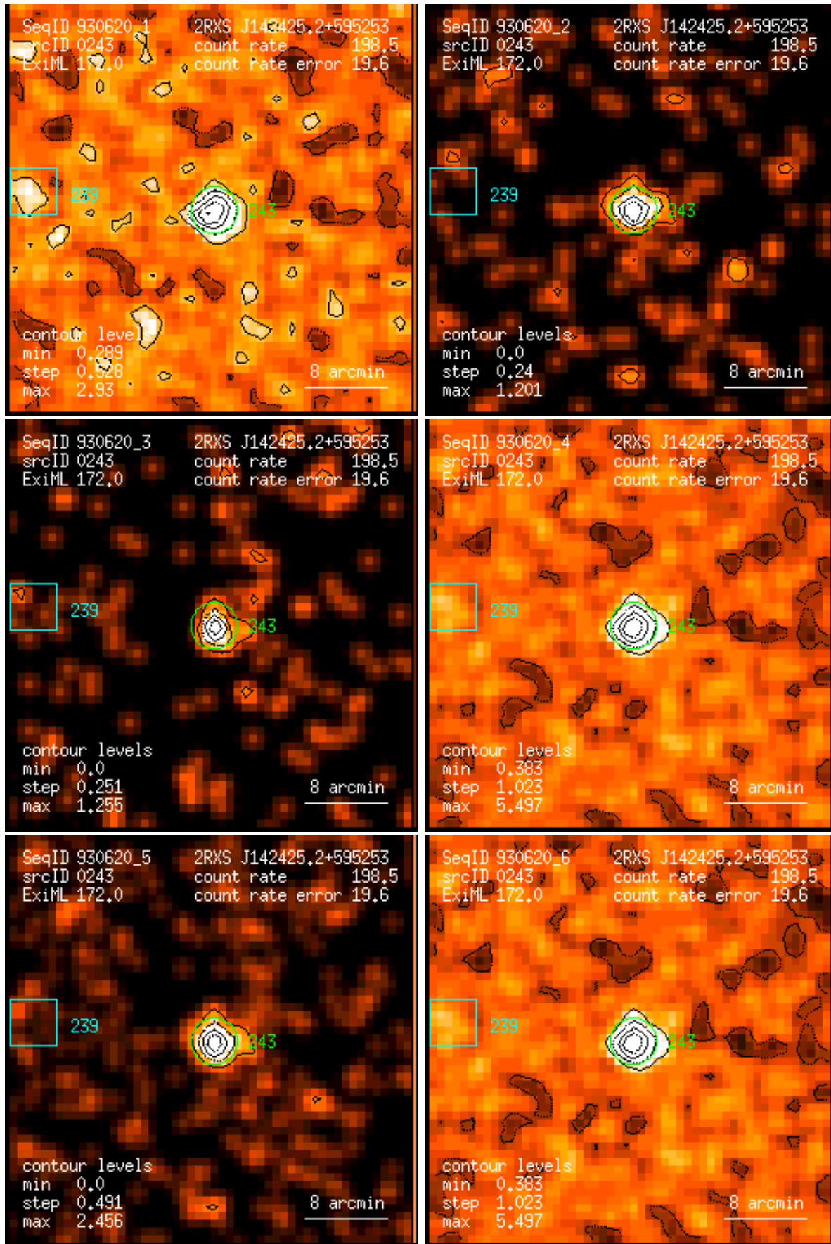
Figure 243: RASS 930620: detection 0243: band rate images, Gaussian filter: (1) PSPC channels 11 – 41, (2) 52 – 90, (3) 91 – 201, (4) 11 – 235, (5) 52 – 201, (6) 11 – 201. Broad band rates in counts/ks. Band rate contour levels in counts/ks/arcmin 2 .
