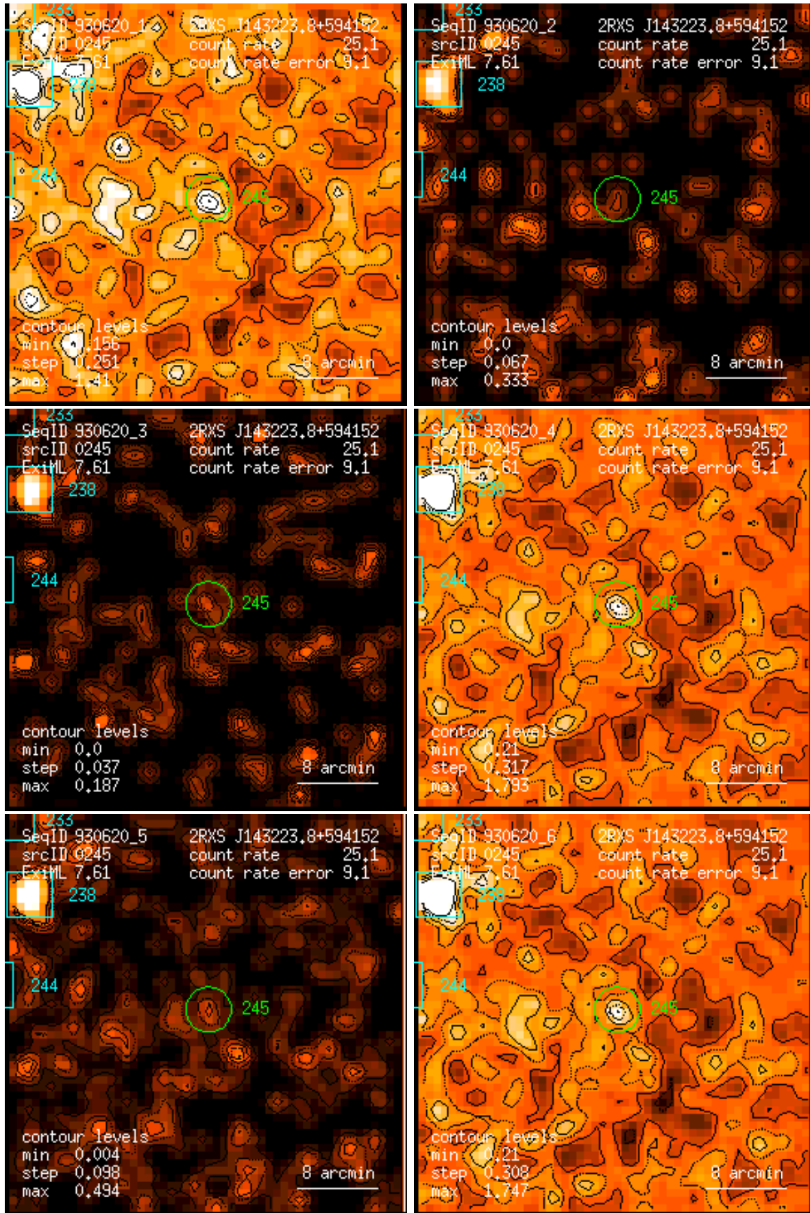
Figure 245: RASS 930620: detection 0245: band rate images, Gaussian filter: (1) PSPC channels 11 – 41, (2) 52 – 90, (3) 91 – 201, (4) 11 – 235, (5) 52 – 201, (6) 11 – 201. Broad band rates in counts/ks. Band rate contour levels in counts/ks/arcmin 2 .
