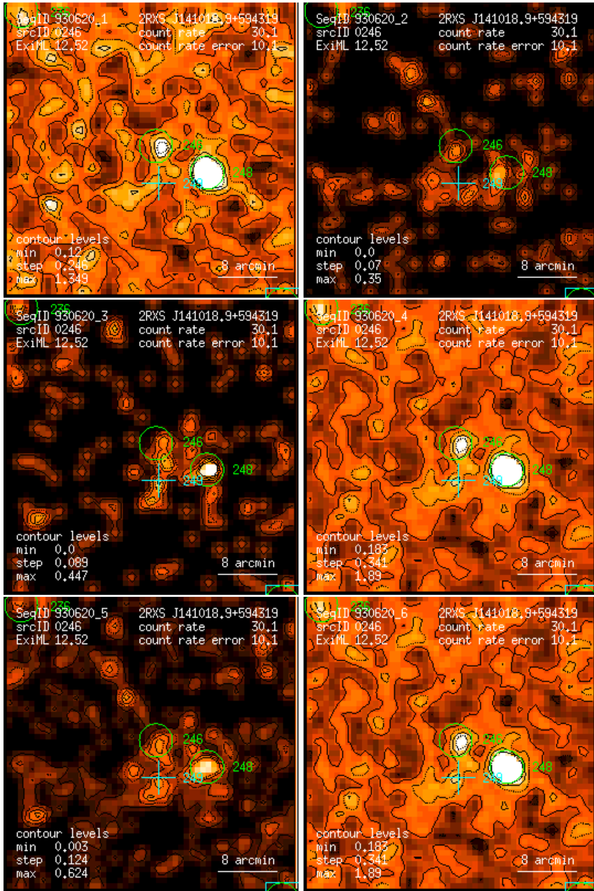
Figure 246: RASS 930620: detection 0246: band rate images, Gaussian filter: (1) PSPC channels 11 – 41, (2) 52 – 90, (3) 91 – 201, (4) 11 – 235, (5) 52 – 201, (6) 11 – 201. Broad band rates in counts/ks. Band rate contour levels in counts/ks/arcmin 2 .
