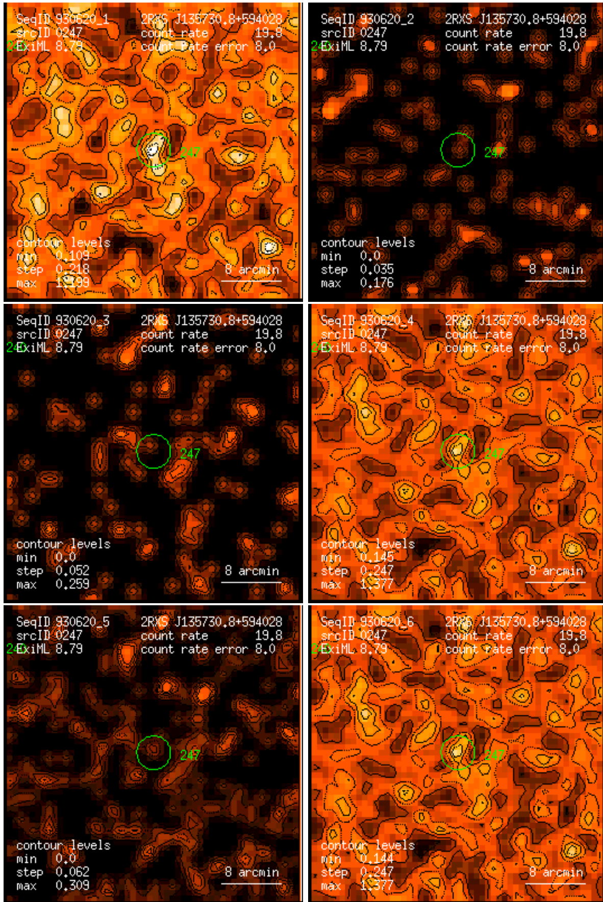
Figure 247: RASS 930620: detection 0247: band rate images, Gaussian filter: (1) PSPC channels 11 – 41, (2) 52 – 90, (3) 91 – 201, (4) 11 – 235, (5) 52 – 201, (6) 11 – 201. Broad band rates in counts/ks. Band rate contour levels in counts/ks/arcmin 2 .
