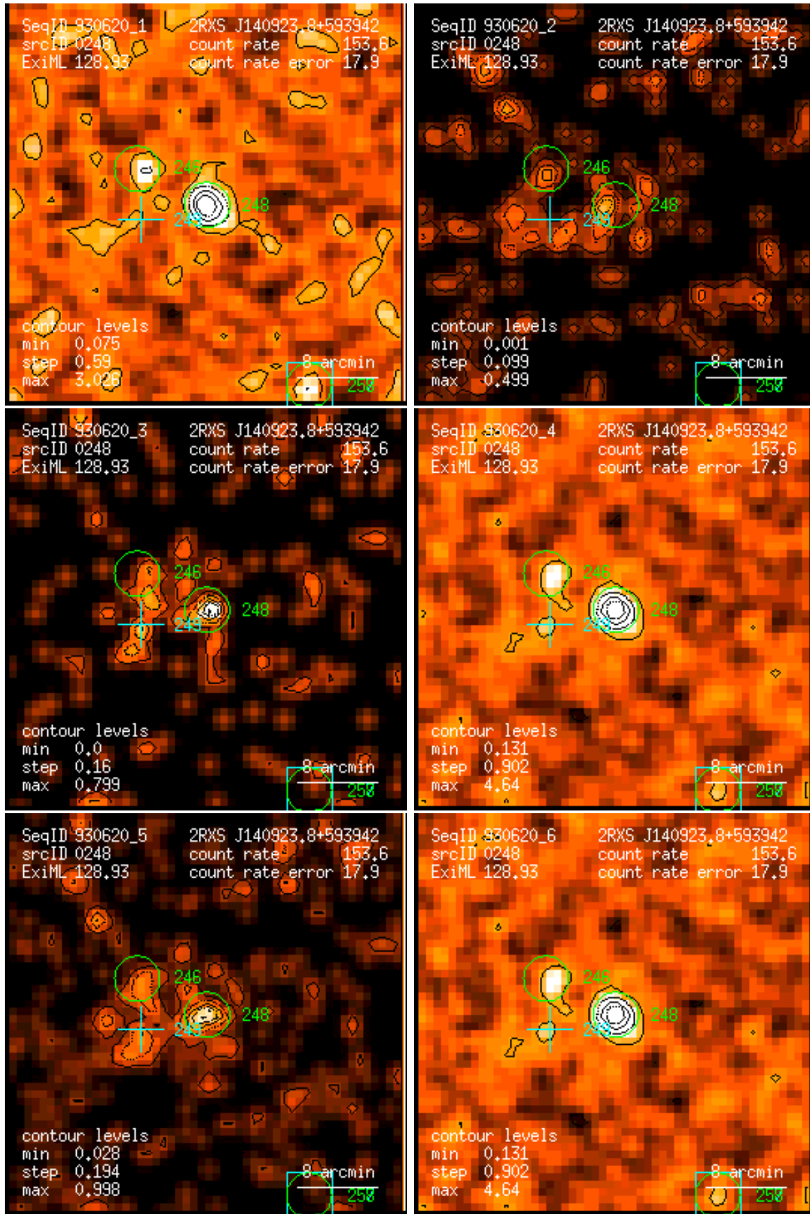
Figure 248: RASS 930620: detection 0248: band rate images, Gaussian filter: (1) PSPC channels 11 – 41, (2) 52 – 90, (3) 91 – 201, (4) 11 – 235, (5) 52 – 201, (6) 11 – 201. Broad band rates in counts/ks. Band rate contour levels in counts/ks/arcmin 2 .
