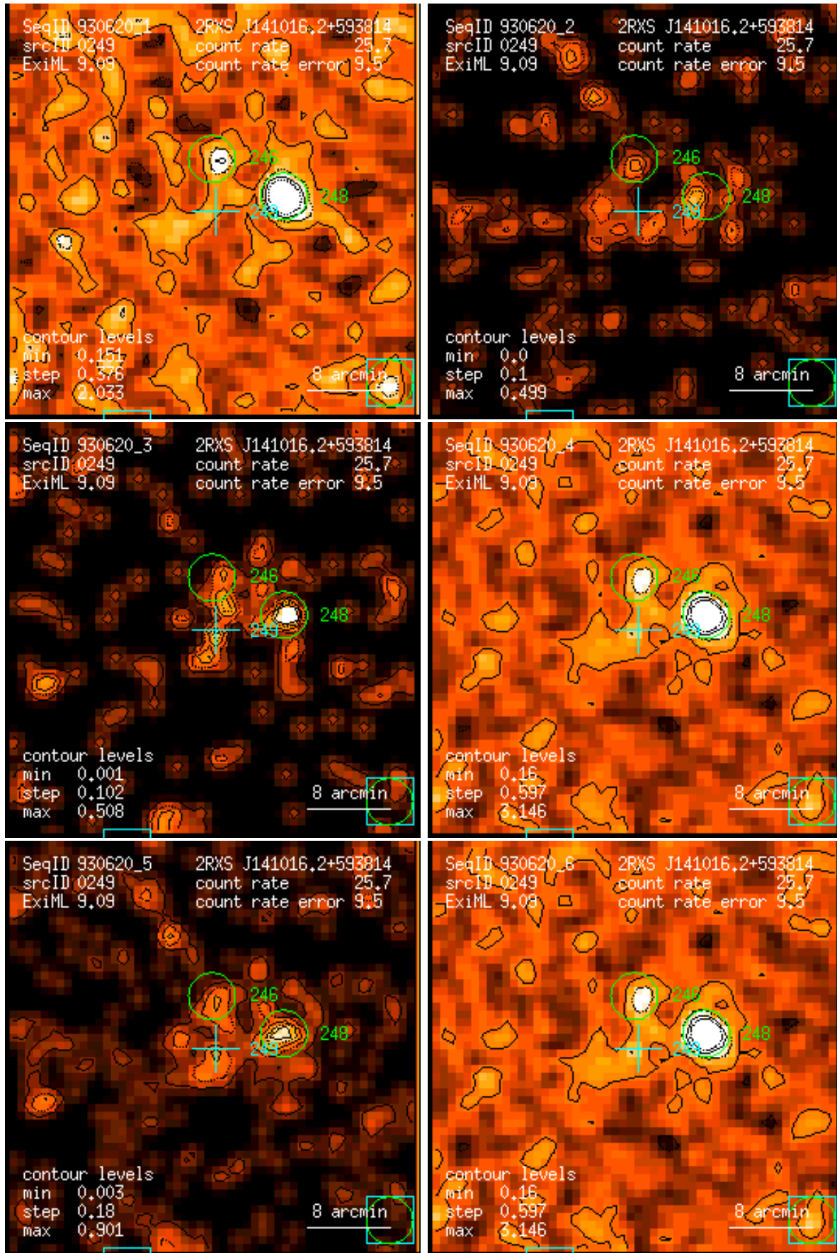
Figure 249: RASS 930620: detection 0249: band rate images, Gaussian filter: (1) PSPC channels 11 – 41, (2) 52 – 90, (3) 91 – 201, (4) 11 – 235, (5) 52 – 201, (6) 11 – 201. Broad band rates in counts/ks. Band rate contour levels in counts/ks/arcmin 2 .
