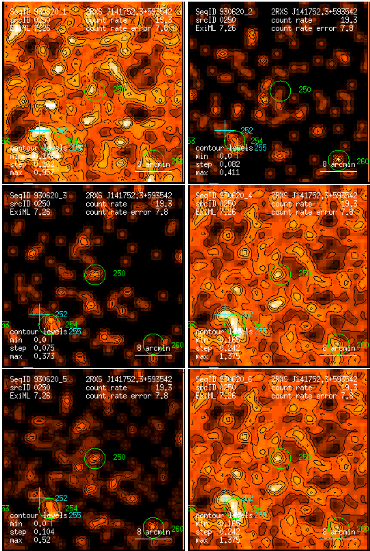
Figure 250: RASS 930620: detection 0250: band rate images, Gaussian filter: (1) PSPC channels 11 – 41, (2) 52 – 90, (3) 91 – 201, (4) 11 – 235, (5) 52 – 201, (6) 11 – 201. Broad band rates in counts/ks. Band rate contour levels in counts/ks/arcmin 2 .
