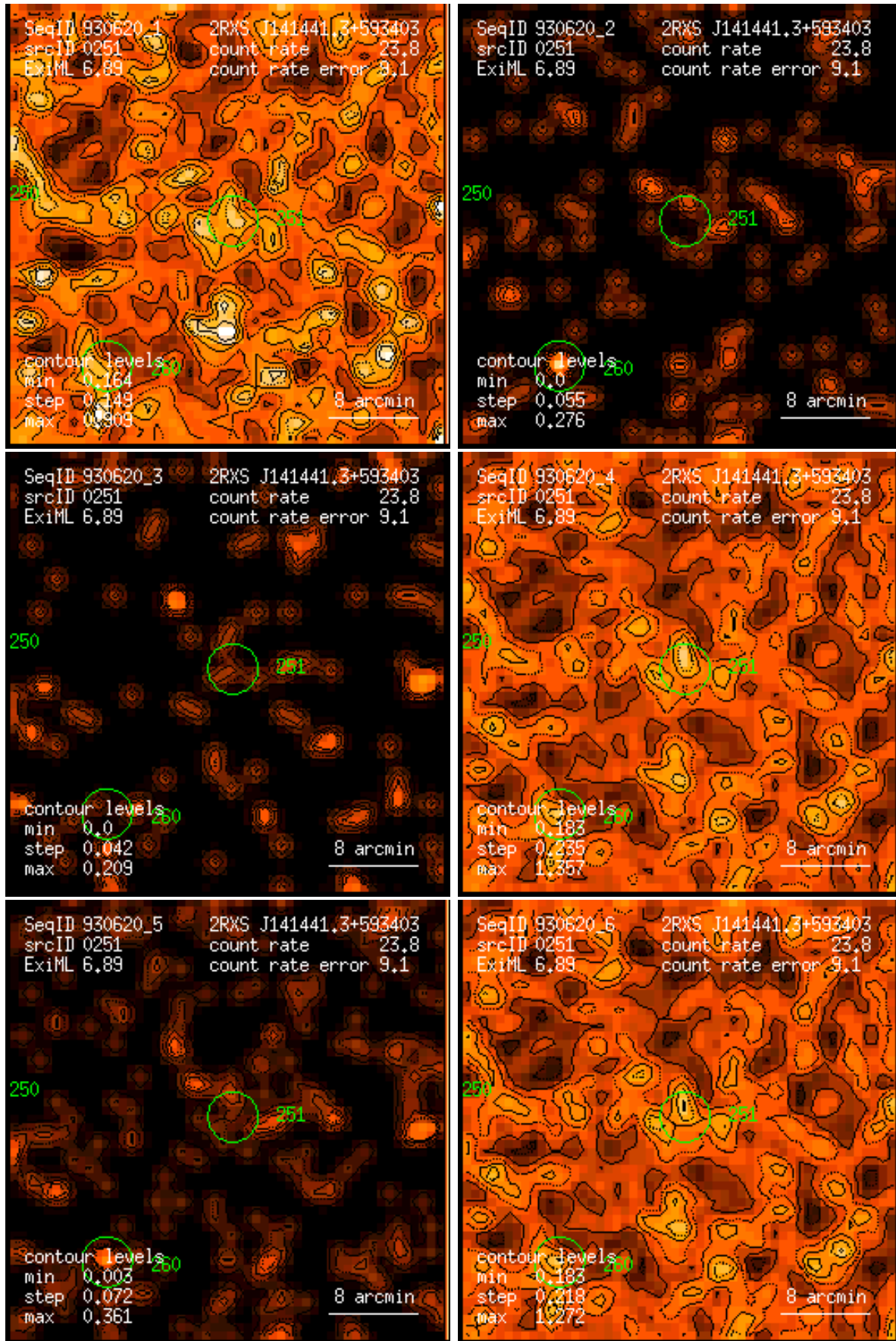
Figure 251: RASS 930620: detection 0251: band rate images, Gaussian filter: (1) PSPC channels 11 – 41, (2) 52 – 90, (3) 91 – 201, (4) 11 – 235, (5) 52 – 201, (6) 11 – 201. Broad band rates in counts/ks. Band rate contour levels in counts/ks/arcmin 2 .
