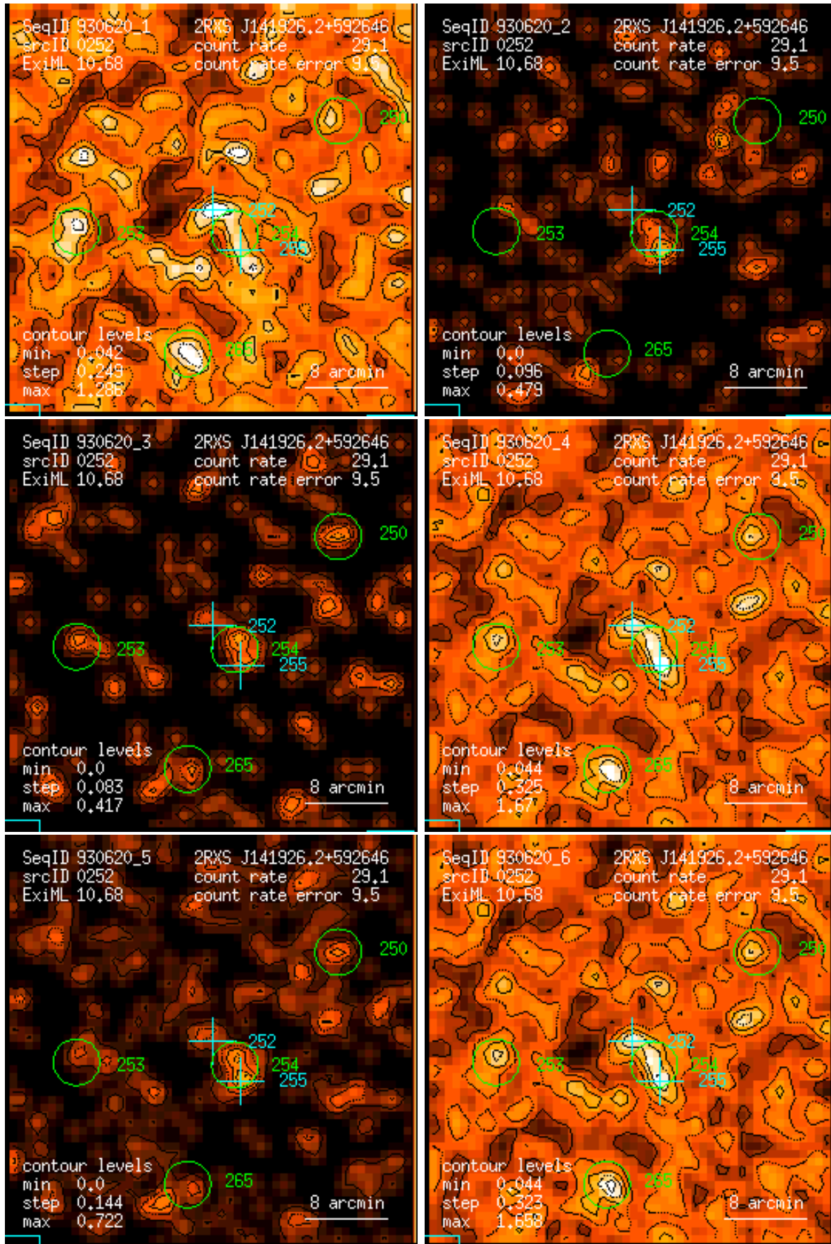
Figure 252: RASS 930620: detection 0252: band rate images, Gaussian filter: (1) PSPC channels 11 – 41, (2) 52 – 90, (3) 91 – 201, (4) 11 – 235, (5) 52 – 201, (6) 11 – 201. Broad band rates in counts/ks. Band rate contour levels in counts/ks/arcmin 2 .
