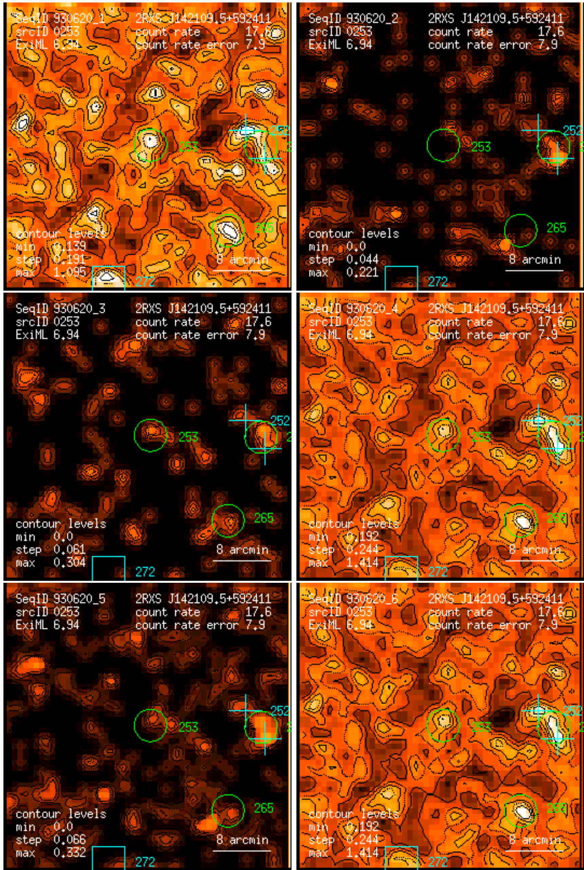
Figure 253: RASS 930620: detection 0253: band rate images, Gaussian filter: (1) PSPC channels 11 – 41, (2) 52 – 90, (3) 91 – 201, (4) 11 – 235, (5) 52 – 201, (6) 11 – 201. Broad band rates in counts/ks. Band rate contour levels in counts/ks/arcmin 2 .
