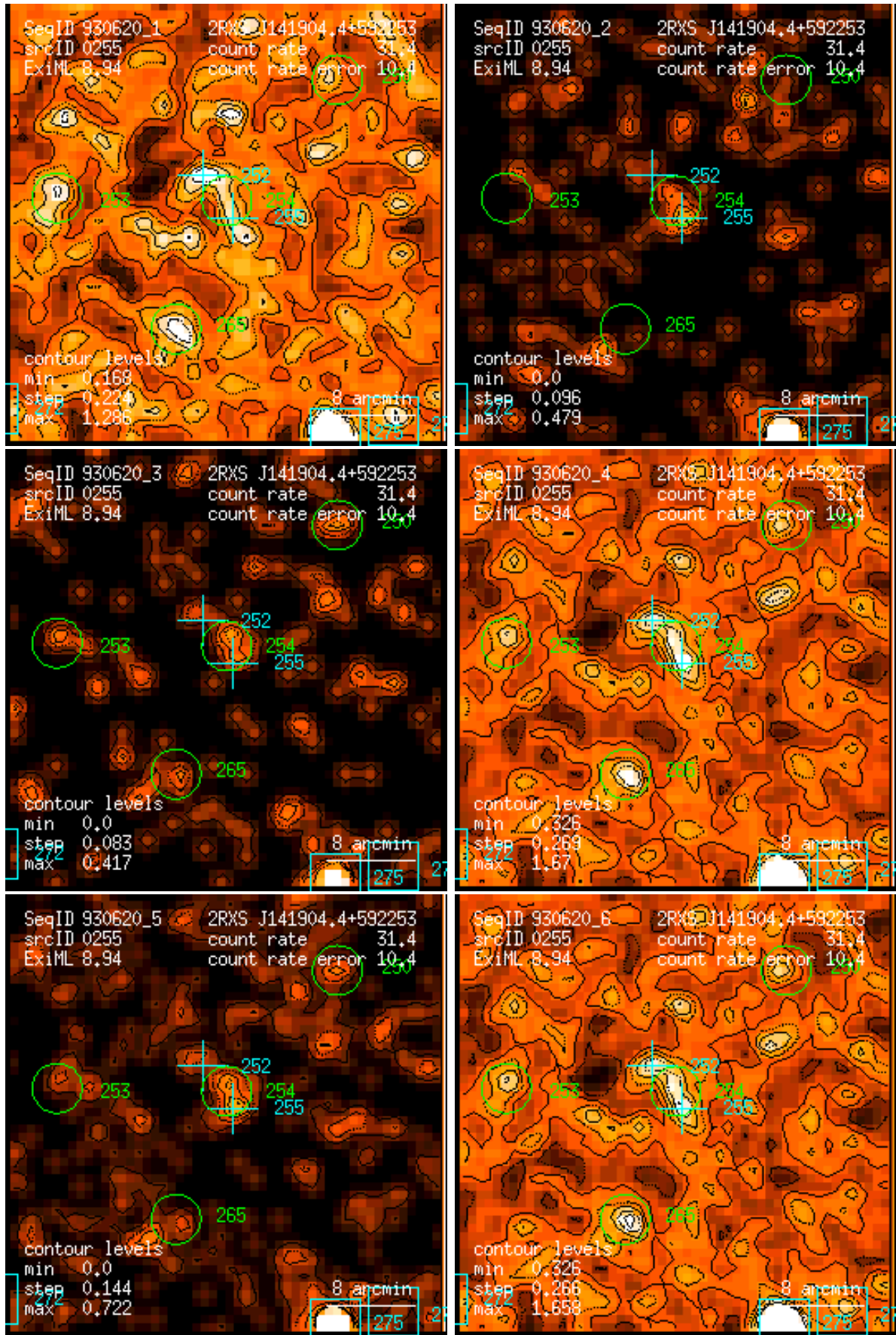
Figure 255: RASS 930620: detection 0255: band rate images, Gaussian filter: (1) PSPC channels 11 – 41, (2) 52 – 90, (3) 91 – 201, (4) 11 – 235, (5) 52 – 201, (6) 11 – 201. Broad band rates in counts/ks. Band rate contour levels in counts/ks/arcmin 2 .
