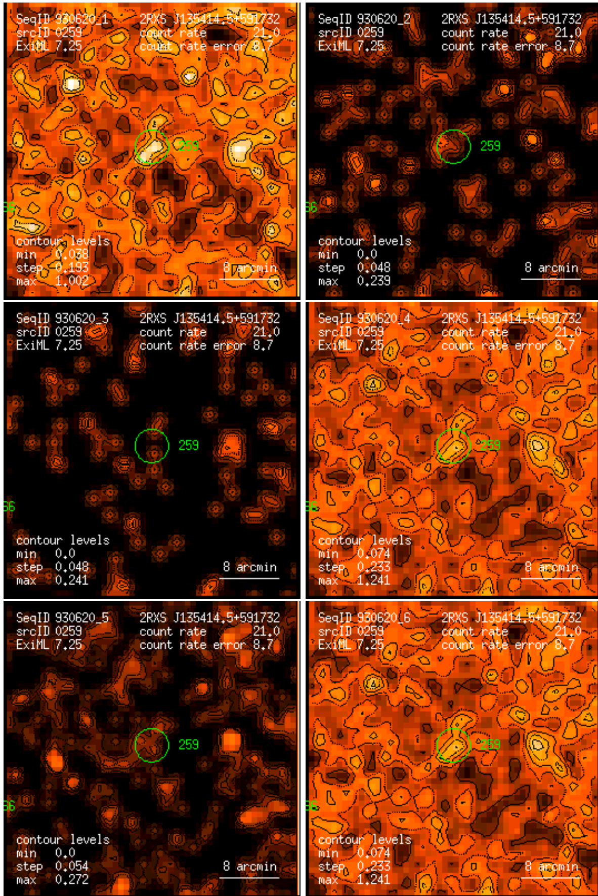
Figure 259: RASS 930620: detection 0259: band rate images, Gaussian filter: (1) PSPC channels 11 – 41, (2) 52 – 90, (3) 91 – 201, (4) 11 – 235, (5) 52 – 201, (6) 11 – 201. Broad band rates in counts/ks. Band rate contour levels in counts/ks/arcmin 2 .
