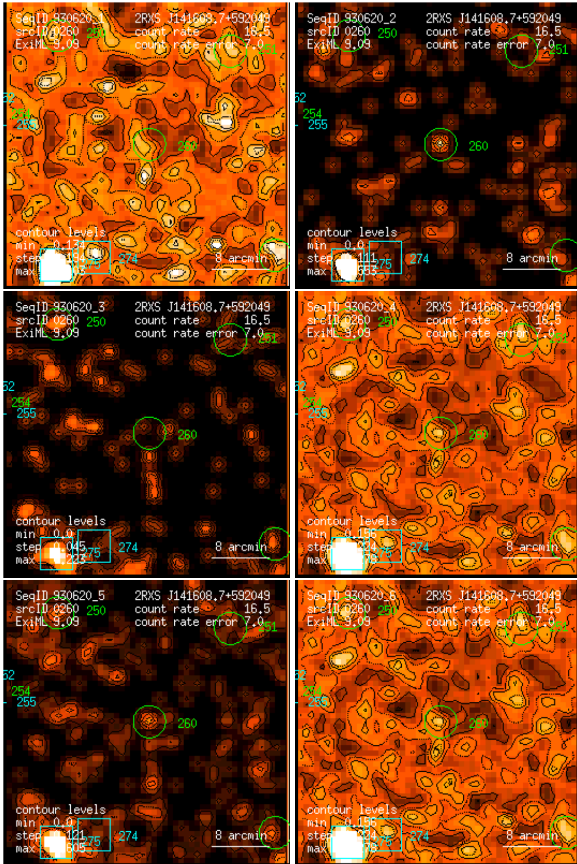
Figure 260: RASS 930620: detection 0260: band rate images, Gaussian filter: (1) PSPC channels 11 – 41, (2) 52 – 90, (3) 91 – 201, (4) 11 – 235, (5) 52 – 201, (6) 11 – 201. Broad band rates in counts/ks. Band rate contour levels in counts/ks/arcmin 2 .
