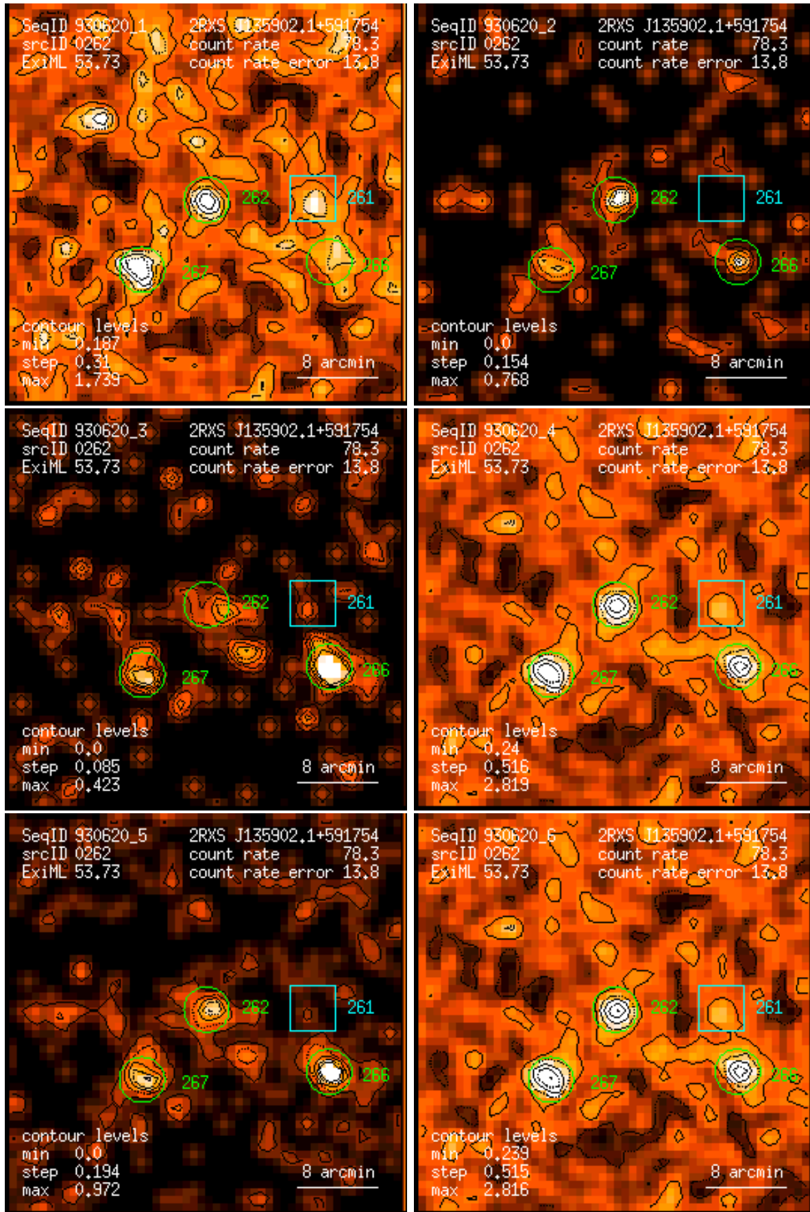
Figure 262: RASS 930620: detection 0262: band rate images, Gaussian filter: (1) PSPC channels 11 – 41, (2) 52 – 90, (3) 91 – 201, (4) 11 – 235, (5) 52 – 201, (6) 11 – 201. Broad band rates in counts/ks. Band rate contour levels in counts/ks/arcmin 2 .
