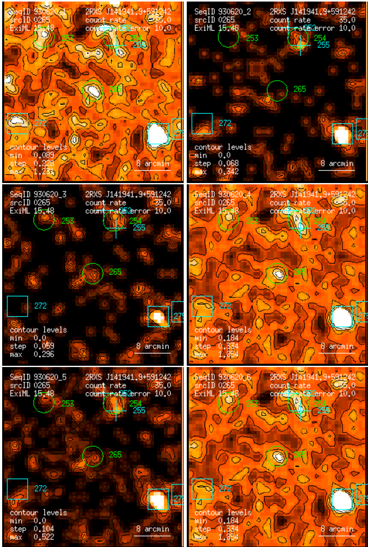
Figure 265: RASS 930620: detection 0265: band rate images, Gaussian filter: (1) PSPC channels 11 – 41, (2) 52 – 90, (3) 91 – 201, (4) 11 – 235, (5) 52 – 201, (6) 11 – 201. Broad band rates in counts/ks. Band rate contour levels in counts/ks/arcmin 2 .
