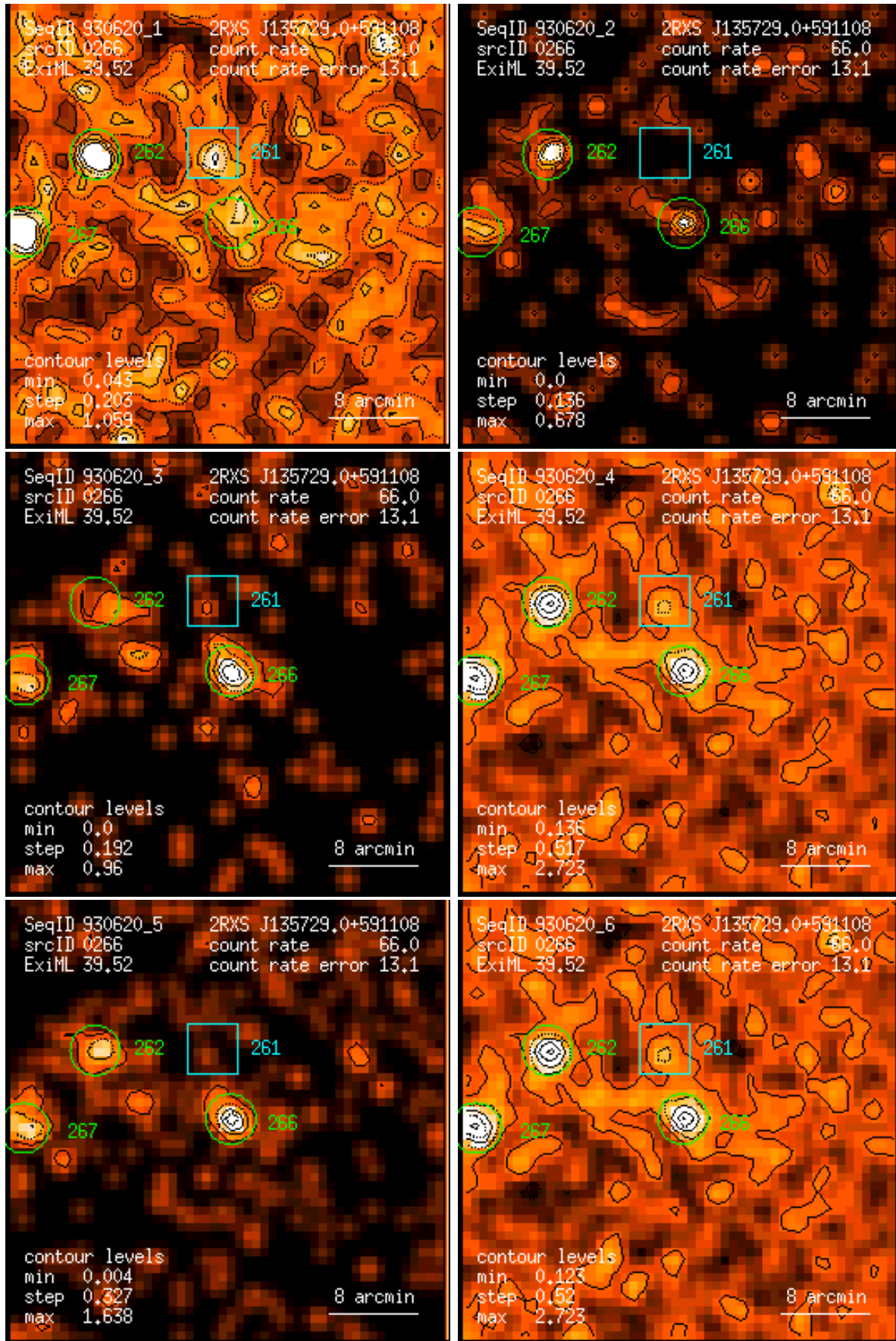
Figure 266: RASS 930620: detection 0266: band rate images, Gaussian filter: (1) PSPC channels 11 – 41, (2) 52 – 90, (3) 91 – 201, (4) 11 – 235, (5) 52 – 201, (6) 11 – 201. Broad band rates in counts/ks. Band rate contour levels in counts/ks/arcmin 2 .
