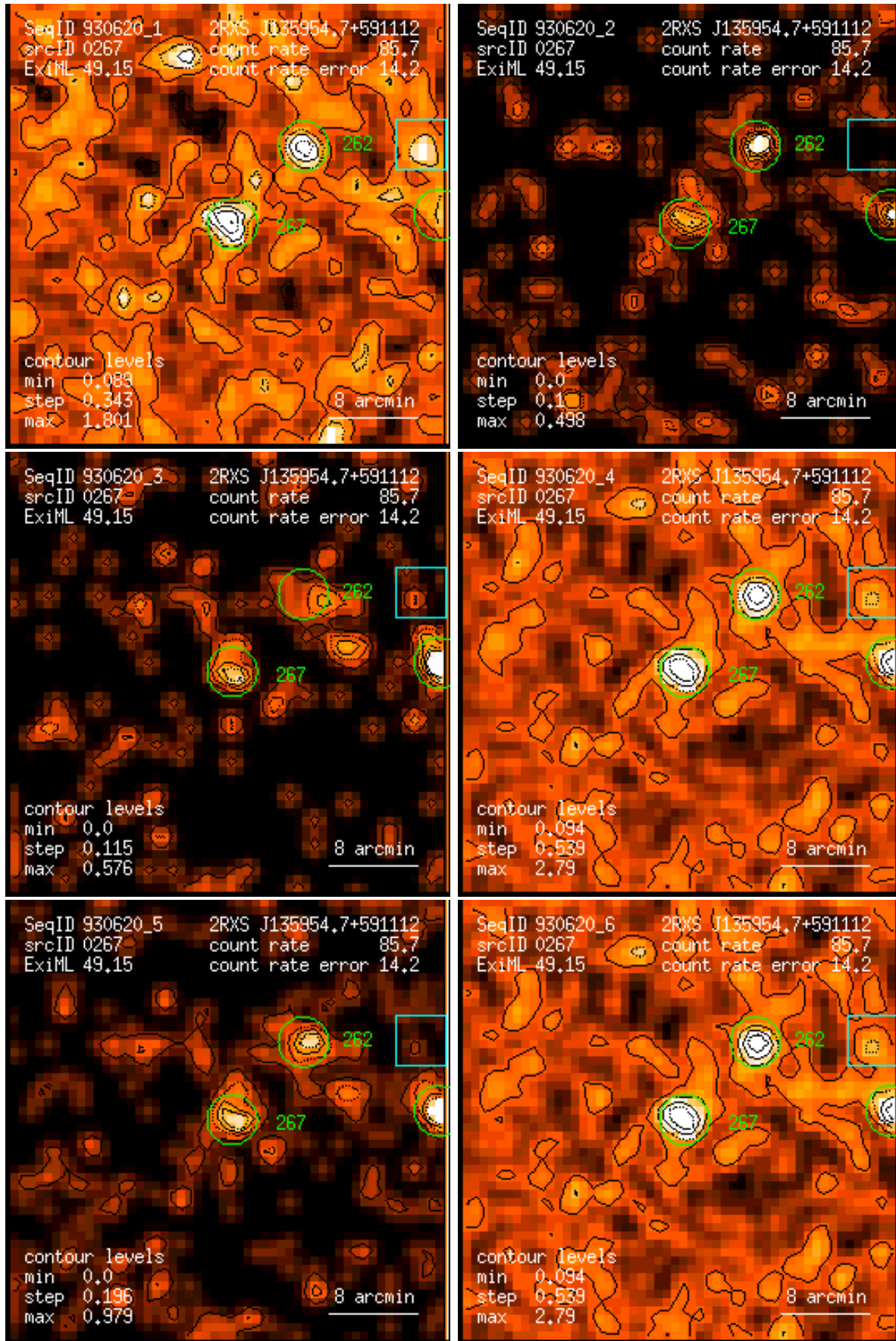
Figure 267: RASS 930620: detection 0267: band rate images, Gaussian filter: (1) PSPC channels 11 – 41, (2) 52 – 90, (3) 91 – 201, (4) 11 – 235, (5) 52 – 201, (6) 11 – 201. Broad band rates in counts/ks. Band rate contour levels in counts/ks/arcmin 2 .
