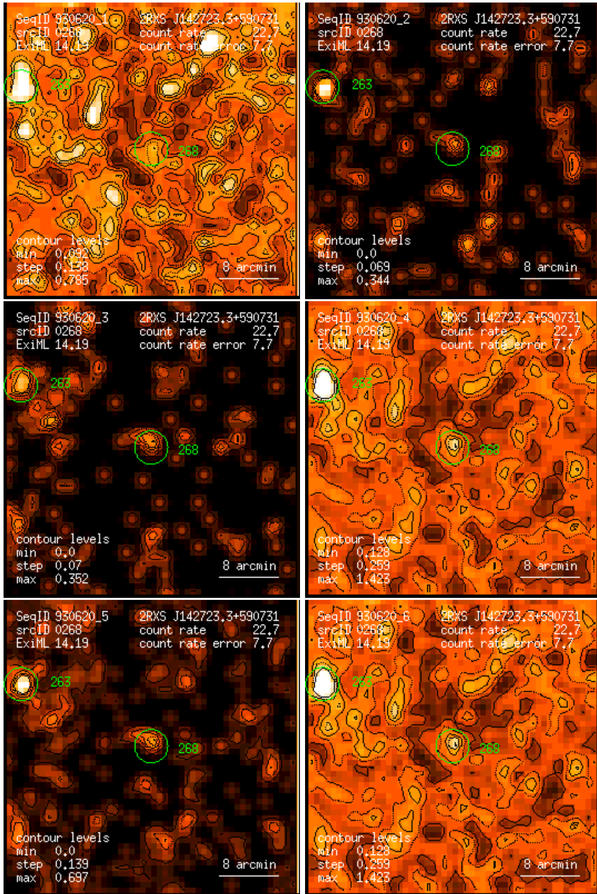
Figure 268: RASS 930620: detection 0268: band rate images, Gaussian filter: (1) PSPC channels 11 – 41, (2) 52 – 90, (3) 91 – 201, (4) 11 – 235, (5) 52 – 201, (6) 11 – 201. Broad band rates in counts/ks. Band rate contour levels in counts/ks/arcmin 2 .
