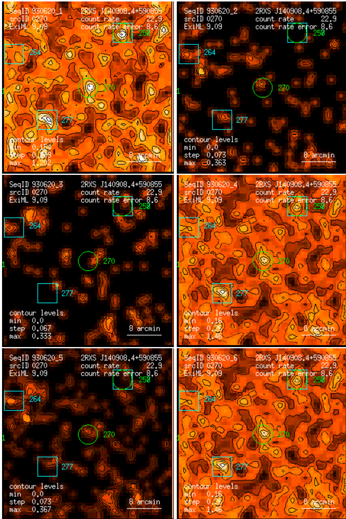
Figure 270: RASS 930620: detection 0270: band rate images, Gaussian filter: (1) PSPC channels 11 – 41, (2) 52 – 90, (3) 91 – 201, (4) 11 – 235, (5) 52 – 201, (6) 11 – 201. Broad band rates in counts/ks. Band rate contour levels in counts/ks/arcmin 2 .
