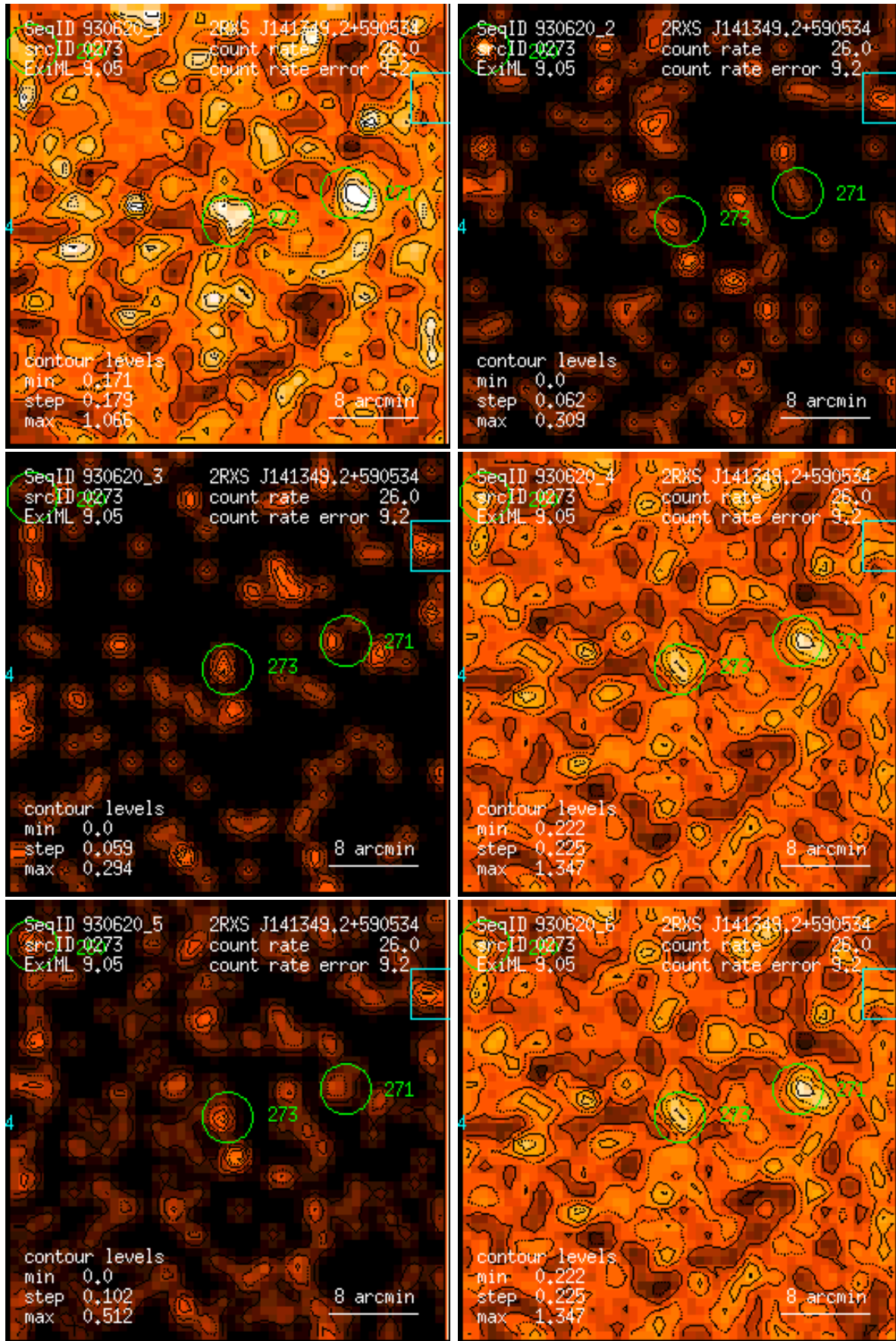
Figure 273: RASS 930620: detection 0273: band rate images, Gaussian filter: (1) PSPC channels 11 – 41, (2) 52 – 90, (3) 91 – 201, (4) 11 – 235, (5) 52 – 201, (6) 11 – 201. Broad band rates in counts/ks. Band rate contour levels in counts/ks/arcmin 2 .
