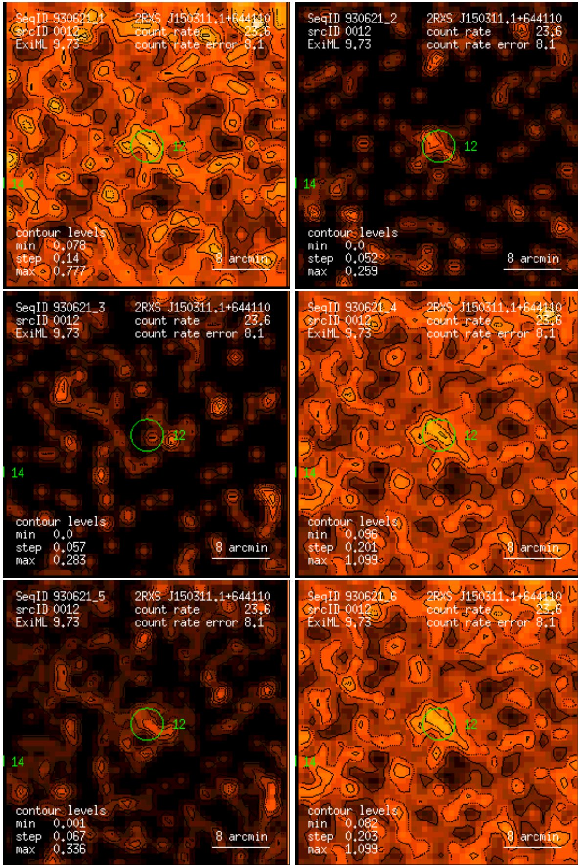
Figure 12: RASS 930621: detection 0012: band rate images, Gaussian filter: (1) PSPC channels 11 – 41, (2) 52 – 90, (3) 91 – 201, (4) 11 – 235, (5) 52 – 201, (6) 11 – 201. Broad band rates in counts/ks. Band rate contour levels in counts/ks/arcmin 2 .
