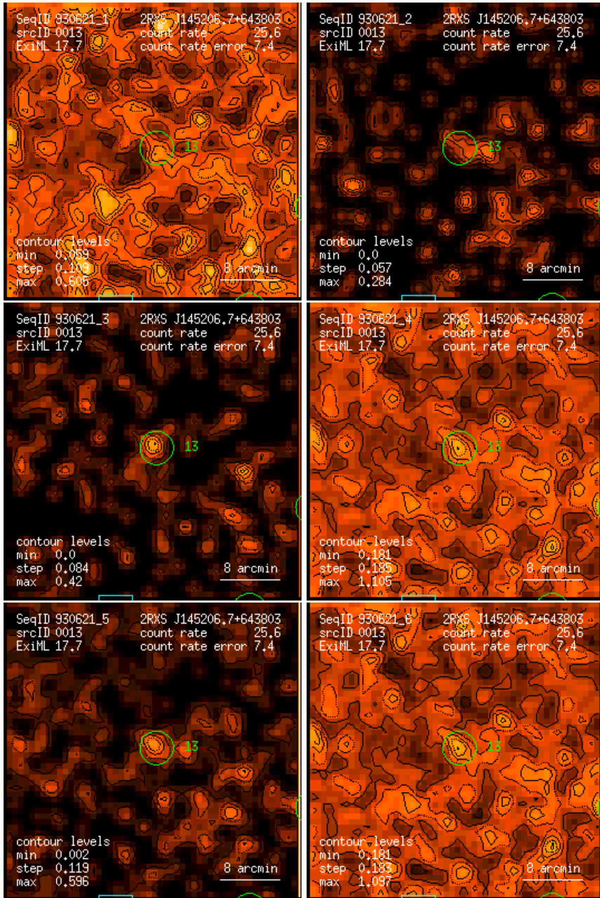
Figure 13: RASS 930621: detection 0013: band rate images, Gaussian filter: (1) PSPC channels 11 – 41, (2) 52 – 90, (3) 91 – 201, (4) 11 – 235, (5) 52 – 201, (6) 11 – 201. Broad band rates in counts/ks. Band rate contour levels in counts/ks/arcmin 2 .
