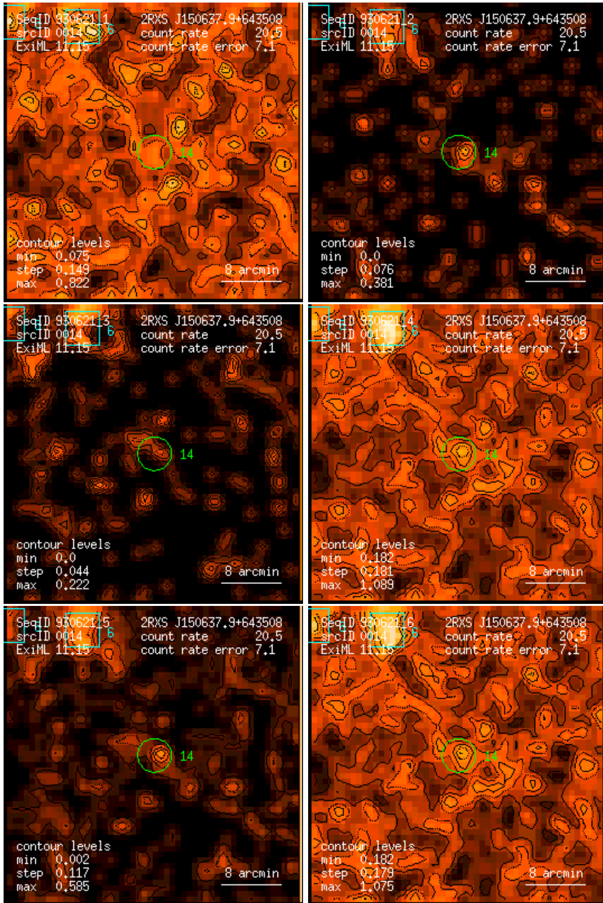
Figure 14: RASS 930621: detection 0014: band rate images, Gaussian filter: (1) PSPC channels 11 – 41, (2) 52 – 90, (3) 91 – 201, (4) 11 – 235, (5) 52 – 201, (6) 11 – 201. Broad band rates in counts/ks. Band rate contour levels in counts/ks/arcmin 2 .
