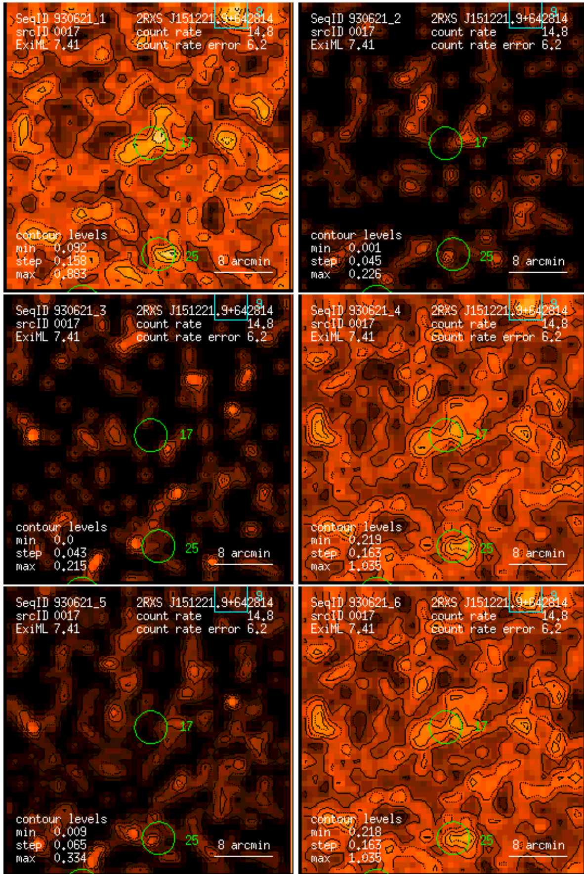
Figure 17: RASS 930621: detection 0017: band rate images, Gaussian filter: (1) PSPC channels 11 – 41, (2) 52 – 90, (3) 91 – 201, (4) 11 – 235, (5) 52 – 201, (6) 11 – 201. Broad band rates in counts/ks. Band rate contour levels in counts/ks/arcmin 2 .
